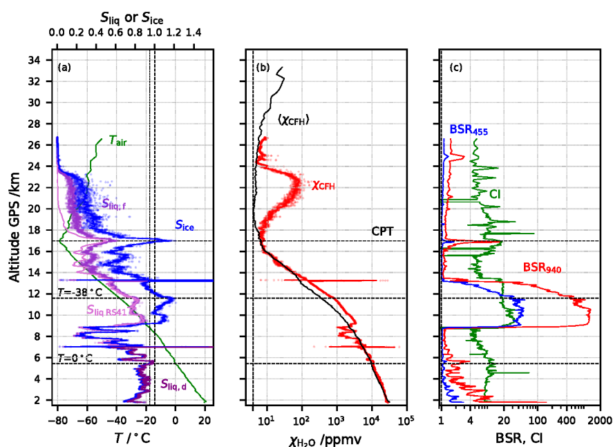
Figure 2. Flight NT011 in Nainital, India, on 15 August 2016. Lines: 1 hPa interval averaged values. Dots: 1 s data. (a) Green: air temperature from Vaisala RS41; pink: saturation over water ( S_{\text{liq,RS41}} ) measured by RS41; blue: ice saturation ( S_{\text{ice}} ) from CFH, dark purple: saturation over water ( S_{\text{liq,d}} ) from CFH considering the deposit on the mirror to be dew; light purple: saturation over water ( S_{\text{liq,f}} ) from CFH considering the deposit on the mirror to be frost. (b) Red: \text{H}_2\text{O} mixing ratio from CFH in ppmv; black: average \text{H}_2\text{O} mixing ratio from uncontaminated CFH for the Nainital 2016 summer campaign (Brunamonti et al., 2018); ‘CPT’ marks the cold point tropopause. (c) Red: 940-nm backscatter ratio from COBALD; blue: same for 455 nm; green: color index (CI) from COBALD.
