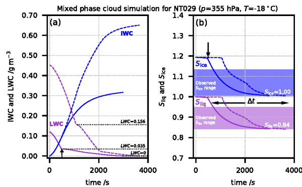
Figure A3. Modelling of the Wegener-Bergeron-Findeisen process in mixed-phase cloud demonstrating that flight NT029 likely encountered supercooled liquid droplets. Solid lines: lower estimate of liquid water content (LWC). Dashed lines: upper estimate (see text). Initial size distributions for lower estimate simulation: n_{ice} = 0.02 \text{ cm}^{-3} , r_{ice} = 10 \text{ }\mu\text{m} ; n_{liq,1} = 20 \text{ cm}^{-3} , r_{liq,1} = 10 \text{ }\mu\text{m} ; n_{liq,2} = 0.002 \text{ cm}^{-3} , r_{liq,2} = 100 \text{ }\mu\text{m} ; n_{liq,3} = 0.001 \text{ cm}^{-3} , r_{liq,3} = 200 \text{ }\mu\text{m} . Initial size distributions for upper estimate simulation are identical but with 3.5\times larger n_{liq,1} and 15\times larger n_{liq,2} . (a) Blue: ice water content (IWC); purple: liquid water content (LWC); vertical arrows: time when smaller liquid droplets fully evaporated. (b) Blue: ice saturation ratio ( S_{ice} ); purple: liquid water saturation ratio ( S_{liq} ) for lower and upper estimates. Glaciation times of small droplets \tau_{g,1} \sim 8 - 18 minutes, of big droplets \tau_{g,2-3} \sim 45 - 50 minutes. Shaded saturation ratios: observed ranges from Figure A2. The computed time interval with S_{ice} and S_{liq} matching flight observations is \Delta t \sim 30 - 40 minutes.
