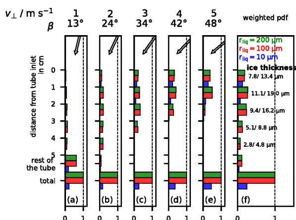
Figure B6. Collision/freezing efficiency of hydrometeors in the intake tube for mixed-phase cloud 1 of flight NT007 with average vertical inlet velocity w_{||} = 4.5 \text{ m s}^{-1} . r_{liq} = 200 \mu m (green), r_{liq} = 100 \mu m (red), r_{liq} = 10 \mu m (blue). (a-e) Freezing efficiency for various velocities ( v_{\perp} ) perpendicular to the tube walls: (a) 1 \text{ m s}^{-1} , 13^{\circ} ; (b) 2 \text{ m s}^{-1} , 24^{\circ} ; (c) 3 \text{ m s}^{-1} , 34^{\circ} ; (d) 4 \text{ m s}^{-1} , 42^{\circ} ; (e) 5 \text{ m s}^{-1} , 48^{\circ} . The ‘rest of the tube’ takes account of all collisions occurring deeper than 5 cm inside the tube, including the mirror holder. (f) Weighted sum of the efficiencies in panels (a-e) by the horizontal velocity pdf of Figure B5a, in front of each bar we write the thickness of the subsequent ice layer considering radial homogeneous cover of the intake tube and the lower (left) and upper (right) LWC estimate for the cloud.
