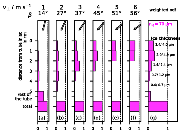
Figure B7. Collision/freezing efficiency of hydrometeors in the intake tube for mixed-phase cloud 2 of flight NT007 with average vertical inlet velocity w_{||} = 4.0 \text{ m s}^{-1} . r_{liq} = 70 \text{ }\mu\text{m} (pink). (a-f) Freezing efficiency for various velocities ( v_{\perp} ) perpendicular to the tube walls: (a) 1 \text{ m s}^{-1} , 14^{\circ} ; (b) 2 \text{ m s}^{-1} , 27^{\circ} ; (c) 3 \text{ m s}^{-1} , 37^{\circ} ; (d) 4 \text{ m s}^{-1} , 45^{\circ} ; (e) 5 \text{ m s}^{-1} , 51^{\circ} ; (f) 6 \text{ m s}^{-1} , 56^{\circ} . The ‘rest of the tube’ takes account of all collisions occurring deeper than 5 cm inside the tube, including the mirror holder. (g) Weighted sum of the efficiencies in panels (a-f) by the horizontal velocity pdf of Figure B5d, in front of each bar we write the thickness of the subsequent ice layer considering radial homogeneous cover of the intake tube and the lower (left) and upper (right) LWC estimate for the cloud.
