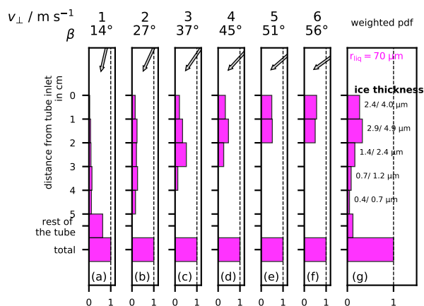
Figure B7. Collision/freezing efficiency of hydrometeors in the intake tube for mixed-phase cloud 2 of flight NT007 with average vertical inlet velocity w_{\parallel} = 4.0 \text{ m s}^{-1} . r_{\text{liq}} = 70 \text{ }\mu\text{m} (pink). (a-f) Freezing efficiency for various velocities ( v_{\perp} ) perpendicular to the tube walls: (a) 1 \text{ m s}^{-1} , 14^{\circ} ; (b) 2 \text{ m s}^{-1} , 27^{\circ} ; (c) 3 \text{ m s}^{-1} , 37^{\circ} ; (d) 4 \text{ m s}^{-1} , 45^{\circ} ; (e) 5 \text{ m s}^{-1} , 51^{\circ} ; (f) 6 \text{ m s}^{-1} , 56^{\circ} . The ‘rest of the tube’ takes account of all collisions occurring deeper than 5 cm inside the tube, including the mirror holder. (g) Weighted sum of the efficiencies in panels (a-f) by the horizontal velocity pdf of Figure B5d, in front of each bar we write the thickness of the subsequent ice layer considering radial homogeneous cover of the intake tube and the lower (left) and upper (right) LWC estimate for the cloud.
