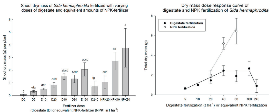
Fig 1. (a) Total shoot drymass of 41 day old Sida hermaphrodita plants fertilized with digestate or equivalent amounts of NPK-fertilizer; bars indicate the standard deviation of the mean (n=5); variants with the same letter are not significantly different (0.05 level); D0: untreated control; D5–D240: digestate doses of 5–240t ha -1 ; NPK 20–80: equivalent amount of NPK fertilizer corresponding to the digestate doses of 20–80t ha -1 , calculated on the basis of the N-content of digestate. (b) Total drymass of 41 day old Sida hermaphrodita plants fertilized with digestate and equivalent N amounts of NPK-fertilizer; bars indicate the standard deviation of the mean (n=5), dose-response line follows the approach of Liebig [14].
