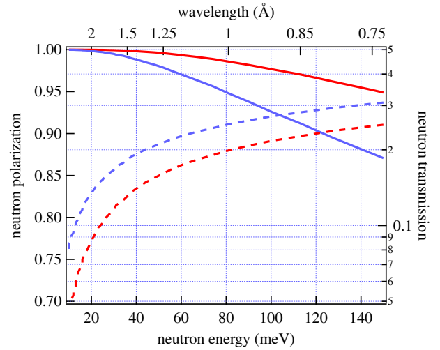
Figure 7. Calculated neutron polarization (solid lines, left axis) and neutron transmission (dashed lines, right axis) with respect to the unpolarized case as a function of neutron energy for the combination of continuously pumped SCF as polarizer and PASTIS layout with wide-angle SFC assuming 75% steady ^3\text{He} polarization for the polarizer and 75% initial ^3\text{He} polarization for the analyzer. The red/blue color corresponds to the individual polarization power of polarizer and analyzer, respectively.
