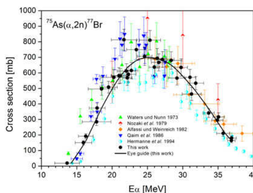
Figure 3. Cross section of the ^{75}\text{As}(\alpha, 2n)^{77}\text{Br} reaction together with literature data [10–14].
