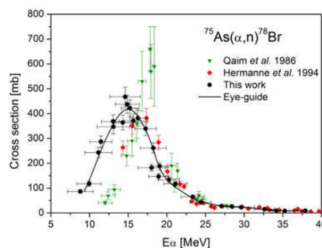
Figure 2. Cross sections of the ^{75}\text{As}(\alpha, n)^{78}\text{Br} reaction together with literature data [10, 11].
