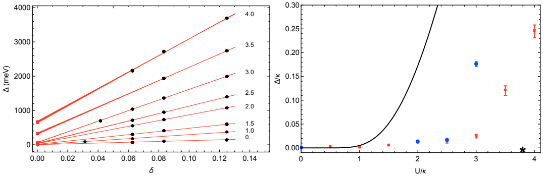
Figure 4. (Left) The dependence of the gap \Delta on \delta = \beta/N_t from the (15,15) tube (black points, error bars too small to be seen), and their continuum extrapolation (red points). The different lines represent calculations with different Hubbard ratios, with the lowest being U/\kappa = 0.5 and highest U/\kappa = 4 , as labelled in the figure. (Right) The dependence of the Mott-insulating gap \Delta (in units of \kappa ) on Hubbard ratio U/\kappa for (15,15) tube (red squares) and (10,10) tube (blue circles). The solid line shows the limiting 1-D analytical result obtained using the Bethe ansatz. Also indicated in the right plot is the location of the critical coupling (black star) for the 2-D hexagonal Hubbard model [12]. The red points of the two plots coincide with each other. [13, 14].
