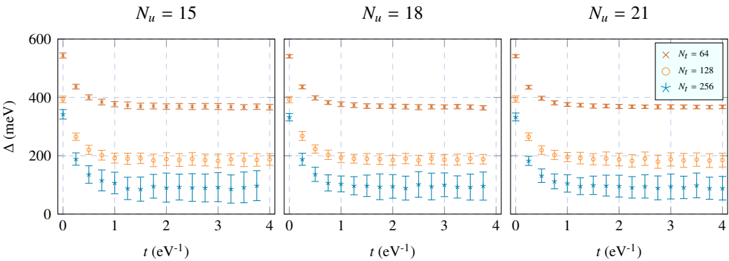
Figure 3. Value of the gap determined from the effective mass at the Dirac point with coupling U/\kappa = 1 and \beta = 8 eV -1 for N_u = 15, 18, 21 and N_t = 64, 128, 256 . Results are nearly independent in N_u for this (weak) value of the coupling, but demonstrate strong dependence on N_t .
