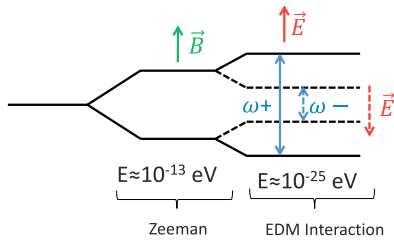
Figure 2. Level scheme ^{129}\text{Xe} -EDM.
