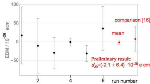
Figure 6. EDM values of different runs.
