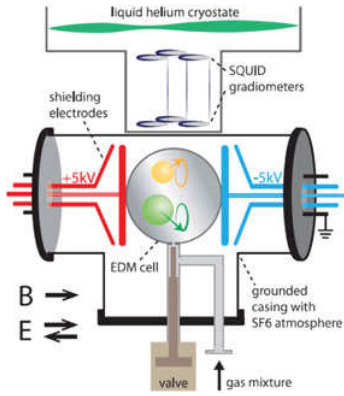
Figure 1. Inner part of the MIXed ^{129}\text{Xe} -EDM experiment.
