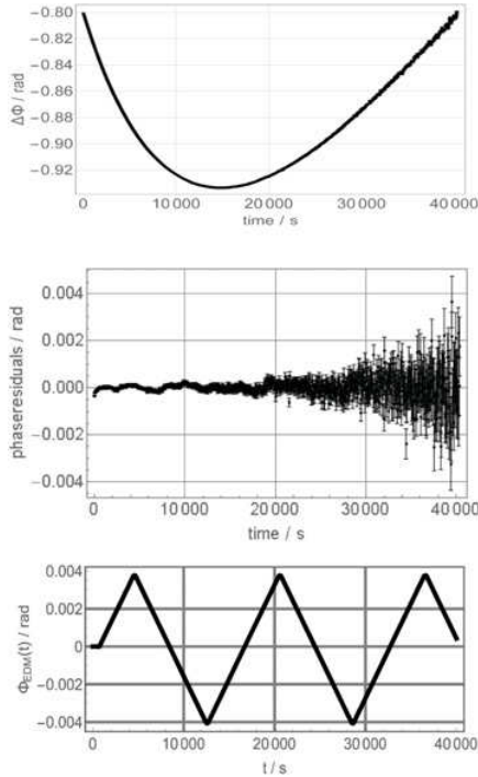
Figure 5. For run number 4; upper part: phase difference \Delta\Phi after correction for earth rotation and chemical shift, middle part: residual phase difference \Delta\Phi after the correction for the generalized Ramsey-Bloch-Siebert-shift, lower part: hypothetical EDM signal \Phi_{EDM}(t) for d_{Xe} = 4.0 \cdot 10^{-25} e \cdot cm .
