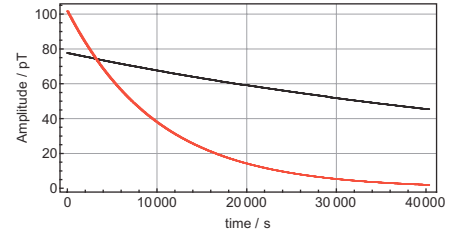
Figure 4. Free induction decay (run number 4) of ^3\text{He} (black) and ^{129}\text{Xe} (red). The error bars are so small and the points are so dense that it looks like continuous lines.
