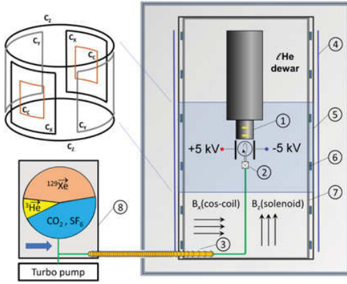
Figure 3. Setup of the MIXed ^{129}\text{Xe} -EDM experiment. The central part of the experiment, i.e. the SQUID-gradiometer (1) and the EDM cell (2), is placed inside a two-layer magnetically shielded room (MSR) with an additional mu-metal cylinder (4) to reduce magnetic field gradients. A coil system consisting of a cosine-coil (5) and a solenoid (6) generates a homogeneous magnetic guiding field. Four additional shimming, coils (shown in the top-left corner) are used to compensate gradients. A fibre-reinforced plastic tube (7) acts a rigid mounting structure for all components inside the MSR. The gas mixture of hyperpolarized ^3\text{He} and ^{129}\text{Xe} , and buffer gases is prepared outside the MSR (8) and then transferred through filling lines equipped with solenoids (3) to the EDM cell.
