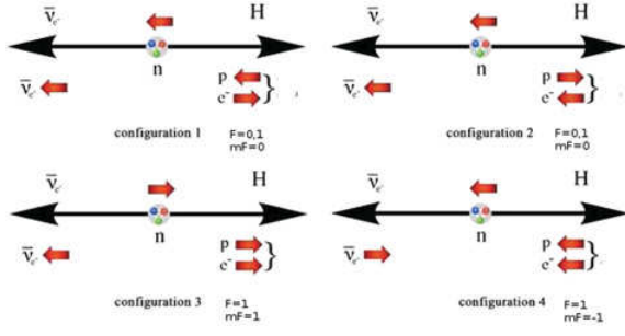
Figure 1. Neutron bound beta decay hydrogen atom hyperfine states (black: momentum, red: spin). Configurations 1, 2, 3 are allowed within the V-A theory. For the configuration 4 a right-handed neutrino is needed. F is the total hyperfine spin and m_F the F projection.
