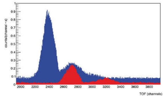
Figure 18. Blue: Secondary electron production by 500 eV protons, accelerated to 18 keV at the foil position in the degrader. Red: Proton (500 eV) distribution at 0 V voltage in the degrader. The proton source \text{H}_2 pressure was 3 \cdot 10^{-3}\text{ mbar} .
