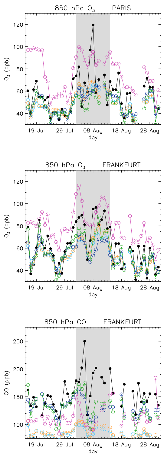
Fig. 4. Time series of daytime average (top) \text{O}_3 above Paris as well as (middle) \text{O}_3 and (bottom) CO above Frankfurt at 850 hPa for the period 15 July–31 August 2003. The area shaded in grey represents the heat wave period (2–14 August). Black lines represent MOZAIC measurements, light blue is used for TM5-HWGL output, orange for TM5-HWHR, dark blue for MOZART, green for MOZART t106 and magenta for MOCAGE.
