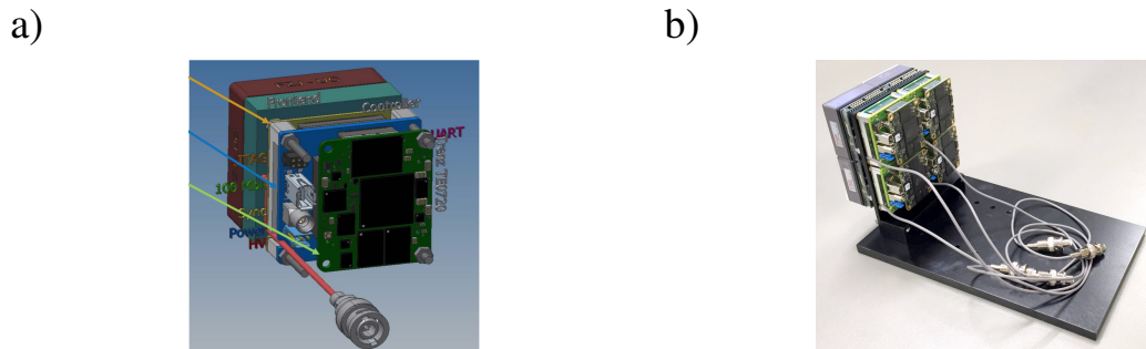
Fig. 4. a) Schematic of a fully assembled SoNDe module. The Trenez module (proprietary FPGA module) containing the FPGA (green), the controller board with ETHERNET, JTAG, LEMO and power connectors (blue) and the front-end board, housing the ASICs (yellow) can all be seen. Between the controller and the front-end board there is an aluminum heat sink, which also protects the bonding wires of the ASICs. The HV cable (red) is channeled past the PCBs. b) Photograph of four fully assembled modules configured in a 2×2 detector array. Edgeless packing allows the construction of large scale detectors with a tiled array.
