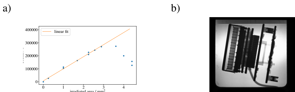
Fig. 5. a) Relation between irradiated area and count-rate. b) Radiograph of the first generation SoNDe Module. It is visible that the boron glass at the front of the MaPMT is nearly intranparent to neutrons. With an additional scintillator in front of the module, the combined shielding effect of the scintillator and the boron glass effectively protect the electronics from radiation damage.
