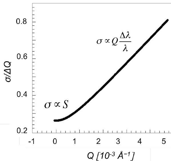
Fig. 5. Q-dependence of the resolution function of KWS3.
