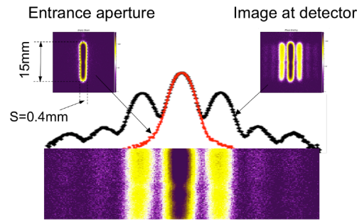
Fig. 3. 1-D diffraction pattern recorded by position sensitive detector.
