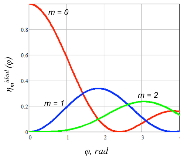
Fig. 6. Diffraction efficiencies of the sinusoidal phase grating.
