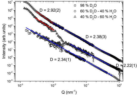
FIG. 4: Small-angle neutron scattering on nuclei of chicken erythrocytes (sample of nuclei fixed in suspension) in heavy water D_2O (chromatin), in 60% D_2O (proteins only) and in 40% D_2O (DNA only).
