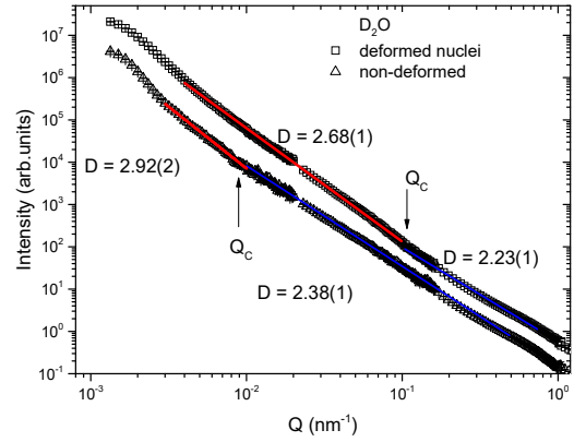
FIG. 5: Small-angle neutron scattering on nuclei of chicken erythrocytes (sample of nuclei deformed (flattened) by centrifugation) in heavy water D_2O (chromatin). The curve for the sample of nuclei fixed in suspension is given in the same picture for comparison.
