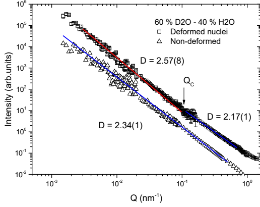
FIG. 6: Small-angle neutron scattering on nuclei of chicken erythrocytes (sample of nuclei deformed (flattened) by centrifugation) in 60% D 2 O (proteins only). The curve for the sample of nuclei fixed in suspension is given in the same pictures for comparison.
