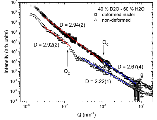
FIG. 7: Small-angle neutron scattering on nuclei of chicken erythrocytes (sample of nuclei deformed (flattened) by centrifugation) in 40% D 2 O (DNA only). The curve for the sample of nuclei fixed in suspension is given in the same pictures for comparison.
