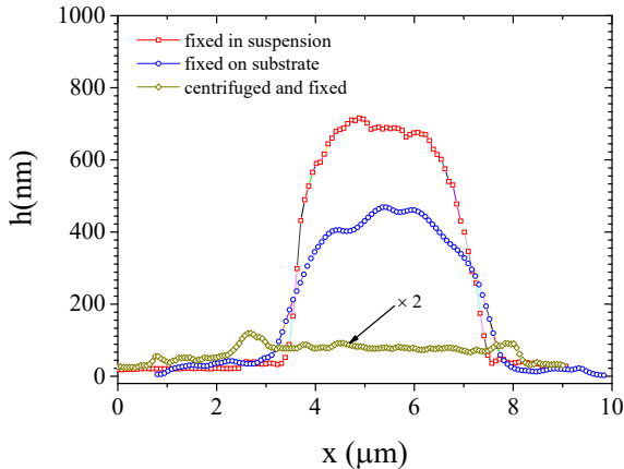
FIG. 3: The cross sections of the surface reliefs of the chicken erythrocytes nuclei shown in Fig.1 for nuclei fixed in suspension, for nuclei fixed on the substrate and for nuclei centrifuged (deformed) and then fixed.
