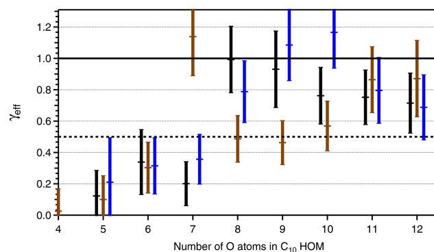
Figure 6. Effective uptake coefficients \gamma_{\text{eff}} for HOM-PPs (C 10 H 14 O x black bars, C 10 H 16 O x , brown bars) and HOM-ONs (C 10 H 15 O x NO 2 , blue bars) as a function of the number of O atoms in the respective HOM. HOMs with different numbers of C, H, and O atoms, e.g., C 10 H y O x and C 9 H y-4 O x+1 HOM-PPs, are treated together, and the number of O atoms is given for the C 10 -HOM-PPs. The second component, C 9 -HOM-PPs, has one O atom more. Data were taken from the β-pinene photooxidation experiment with [β-pinene] SS ~ 10 ppb, [NO x ] SS ~ 4 ppb. The signal intensity for the C 10 H 14 O 4 and HOM-ONs with four O atoms was too low to allow reliable determination of \gamma_{\text{eff}} , and the respective data are left out. Uncertainties in \gamma_{\text{eff}} arise from the determination procedure as shown in Fig. 5. The black line indicates \gamma_{\text{eff}} = 1 and 0.5. An average Fuchs–Sutugin correction factor of 0.70 ( d_p = 175 nm) was applied to calculate \gamma_{\text{eff}} .
