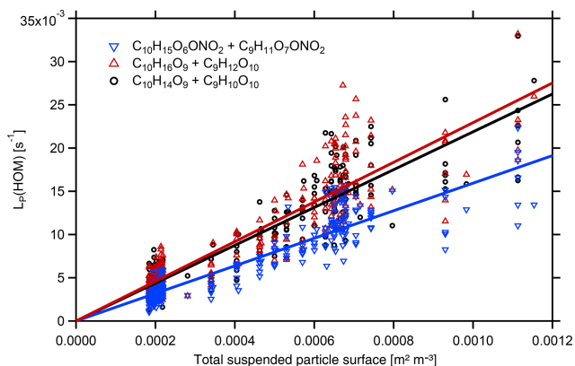
Figure 5. Plot of L_p(\text{HOM}) calculated by Eq. (6) versus particle surface area, S_p , for the examples of HOM-ONs with a molecular mass of = 293 Da (C 10 H 15 O 6 ONO 2 and C 9 H 11 O 7 ONO 2 ), HOM-PPs with a molecular mass of 280 Da (C 10 H 16 O 9 and C 9 H 12 O 10 ), and HOM-PPs with molecular mass of 278 (C 10 H 14 O 9 and C 9 H 10 O 10 ). HOMs from β-pinene photooxidation ([β-pinene] SS ~ 10 ppb, [NO x ] SS ~ 4 ppb). Dividing the slopes by the respective \tilde{v}/4 led to f_{FS} \times \gamma_{\text{eff}} \sim 0.5 for the example HOM-ONs and ~ 0.6 in the latter cases. The main uncertainty arises from the scatter of L_p(\text{HOM}) individual unit mass resolution data. Statistical errors of f_{FS} \times \gamma_{\text{eff}} were about ± 5 %.
