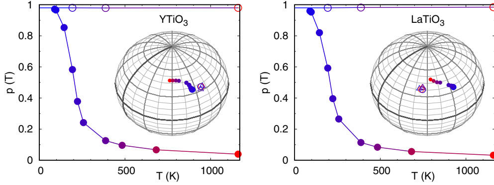
FIG. 4. Superexchange-driven orbital-ordering transition in \text{YTiO}_3 (left) and \text{LaTiO}_3 (right). The plots show the orbital polarization p(T) as a function of temperature. Darker symbols correspond to lower temperatures. For each temperature, the most occupied state, |\vartheta, \varphi\rangle_1 = \sin \vartheta \cos \varphi |xz\rangle_1 + \cos \vartheta |xy\rangle_1 + \sin \vartheta \sin \varphi |yz\rangle_1 , is indicated on the sphere in the inset, where the two dark lines correspond to \vartheta = 90^\circ (equatorial) and \varphi = 0^\circ (vertical). Open circles: LDA+DMFT results with full crystal-field splitting. Solid circles: results in the zero-crystal-field splitting limit. Triangles: lowest-energy crystal-field orbital from LDA calculations for the experimental structure measured at 2 and 293 K for \text{YTiO}_3 (crystal structures from Refs. [11,33]) and 8, 293, and 747 K for \text{LaTiO}_3 (crystal structures from Refs. [11,22]).
