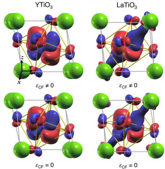
FIG. 5. Top: Lowest-energy crystal-field orbital at site \text{Ti}_1 , |\vartheta_{\text{CF}}, \varphi_{\text{CF}}\rangle . It is very close to the most occupied natural orbital in the presence of the full static crystal-field splitting \epsilon_{\text{CF}} . Bottom: Most occupied natural orbital |\vartheta_{\text{KK}}, \varphi_{\text{KK}}\rangle for idealized structure with no static crystal-field splitting in the T \rightarrow 0 limit. Left: \text{YTiO}_3 . Right: \text{LaTiO}_3 .
