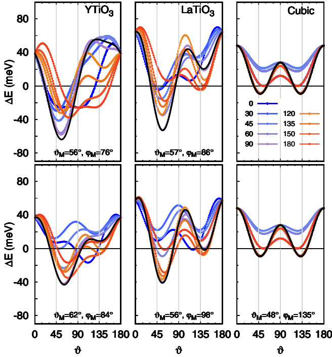
FIG. 6. Superexchange total energy gain \Delta E(\vartheta, \varphi) for a classical orbitally ordered ground state compatible with the GdFeO 3 -type distortion. The energy zero is the energy of the paraorbital state. In each panel, the different lines correspond to the values of \varphi specified in the top right panel. Top: all superexchange terms. Bottom: only quadratic terms. Left: YTiO 3 . Middle: LaTiO 3 . Right: For comparison, we show the result for the cubic case. We chose t \sim 150 meV, which is a value representative for LaTiO 3 and YTiO 3 , see Table I. Black lines: \varphi values that yield the energy minimum, indicated in each case. The results are invariant under the transformation (\vartheta, \varphi) \rightarrow (180^\circ - \vartheta, \varphi - 180^\circ) ; hence, we show only results for \vartheta and \varphi between 0^\circ and 180^\circ . In the cubic limit an additional symmetry is present, (\vartheta, \varphi) \rightarrow (180^\circ - \vartheta, \varphi) .
