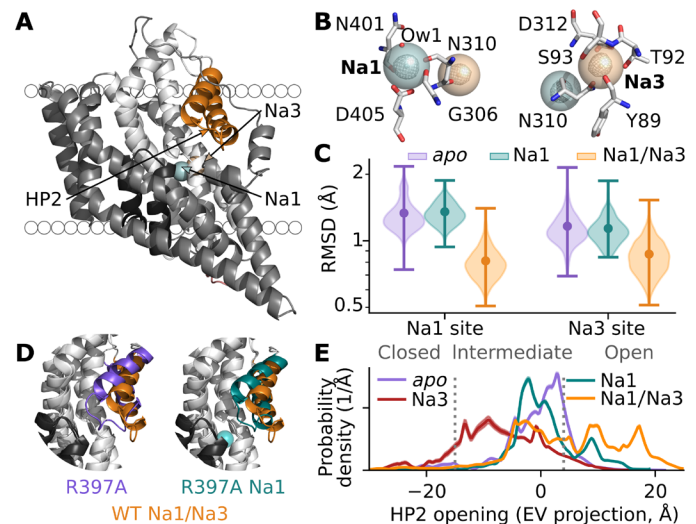
Fig. 2. \text{Glt}_{\text{ph}} crystal structure reveals the Na1/Na3-bound fully open state. (A) X-ray crystal structure of \text{Na}^+ -bound WT \text{Glt}_{\text{ph}} at 2.5-Å resolution in the outward-facing conformation. (B) Close-up images of the occupied Na1 and Na3 sites (gray mesh, omit map contoured at 5.0 \sigma ) and the coordinating residues. (C) Root mean square deviation of binding-site residues from the crystal structure (A) in 60-ns MD simulations with either binding sites occupied or ions manually removed. (D) Superimposition of the \text{Na}^+ -bound WT structure on apo [Protein Data Bank (PDB): 4OYE] or Na1-bound R397A \text{Glt}_{\text{ph}} (PDB: 4OYF) to highlight differences in the HP2 gate. (E) Probability densities for HP2 opening as a function of Na1- and Na3-site occupancies from umbrella sampling simulations (EV, eigenvector).
