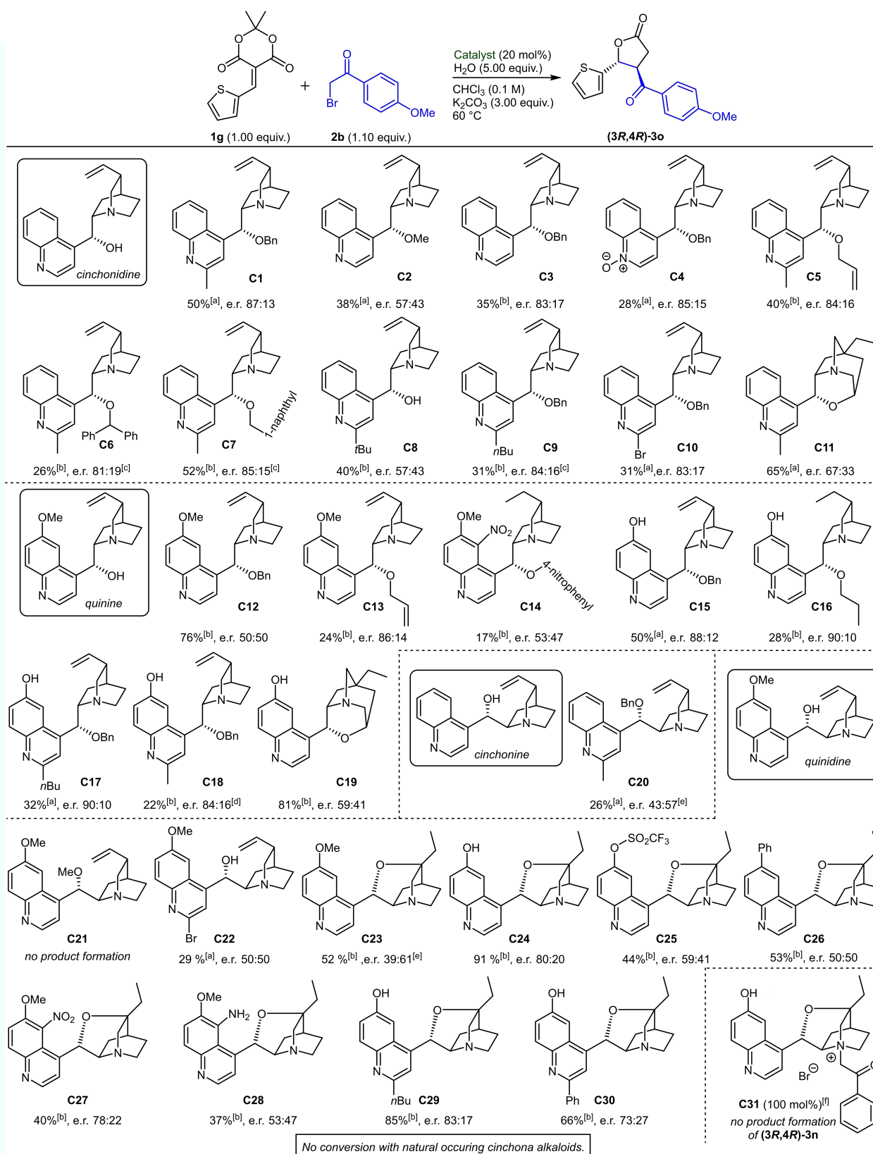
Scheme 5. Enantioselective screening of catalysts C . All reactions were carried out on a 0.10 mmol scale. [a] Yield of isolated product. [b] Quantification via 1 H NMR spectroscopy with DMF as an internal standard. [c] Product obtained with d.r. 3:1 ( trans : cis ). [d] 8.0 mol% catalyst loading. [e] Opposite trans -enantiomer favored. [f] No more \alpha -bromoacetophenone ( 2a ) was added.
