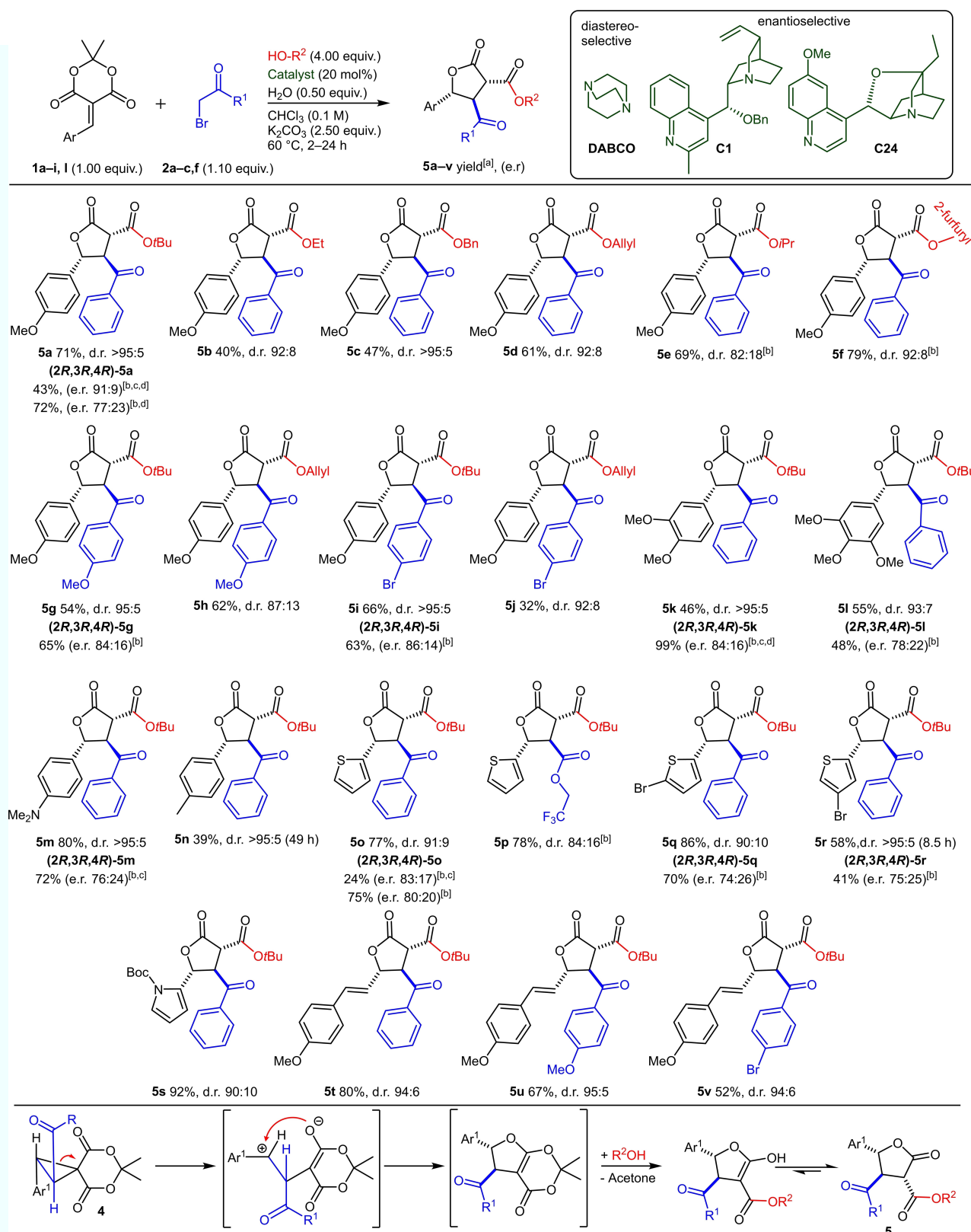
Scheme 7. Above) Scope of the all-trans - \alpha,\beta,\gamma -substituted \gamma -butyrolactone 5 synthesis. Diastereoselective reactions were conducted on a 0.25 mmol scale. For the enantioselective transformation, C24 was employed. [a] Yield of isolated product. [b] Reaction was carried out on a 0.10 mmol scale. [c] Reaction was catalyzed with C1 . [d] e.r. determined after decarboxylation of malonic ester. Below) Proposed mechanism of \alpha,\beta,\gamma -substituted butyrolactone 5 formation.
