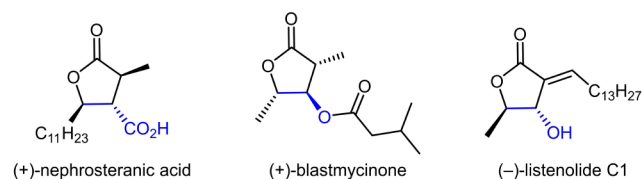
Figure 1. Selected examples of trans - \gamma -butyrolactone-containing natural products.
