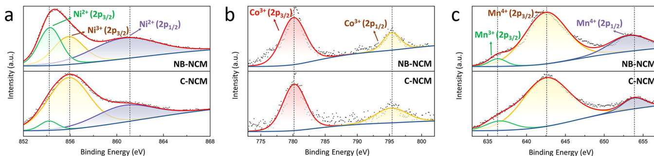
Figure 3. XPS spectra of (a) Ni 2p, (b) Co 2p, and (c) Mn 2p in as-prepared NB-NCM (upper curves) and C-NCM (lower curves).
