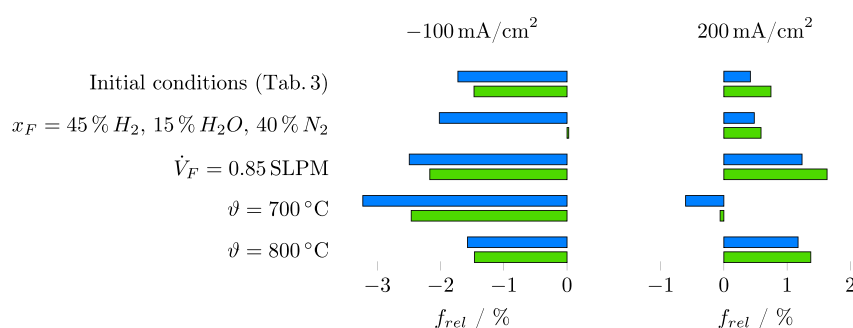
Fig. 11 – Comparison of relative error between the simulated and measured cell voltage in both electrolysis and fuel cell mode for transfer coefficients of ■ 0.75 and ■ 0.85 when varying operating conditions.
