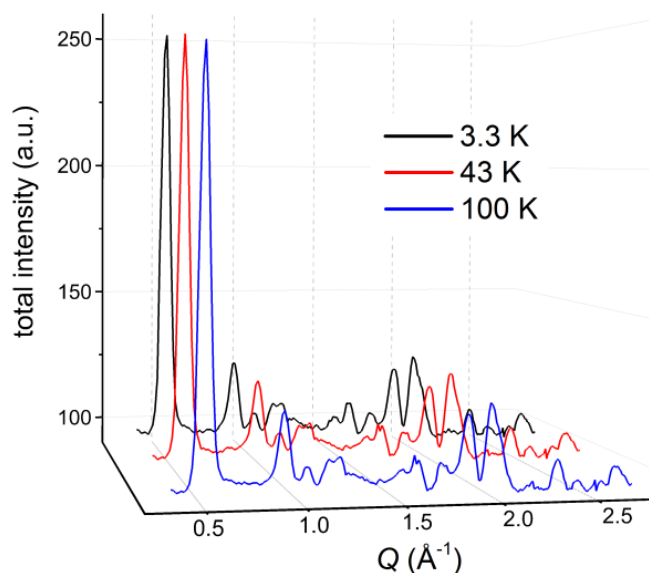
Figure 8. Total neutron scattering intensity measured on DNS at 3.3, 43, and 100 K.
