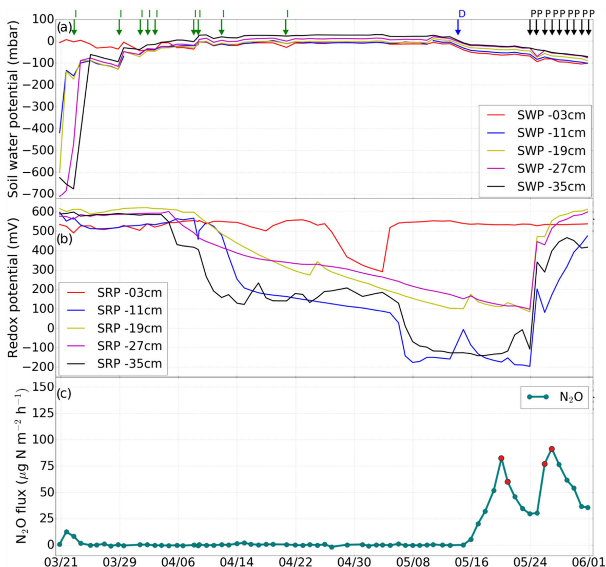
Figure 2. Experiment 1 (before fertilization). Changes in (a) soil water potential (SWP), (b) soil redox potential (SRP), and (c) N_2O emission rate induced by irrigation (I), drainage (D), irrigation with fertilizer (F), desaturation of the soil with pump (P). The red dots in panel c indicate the N_2O isotope sampling days.
