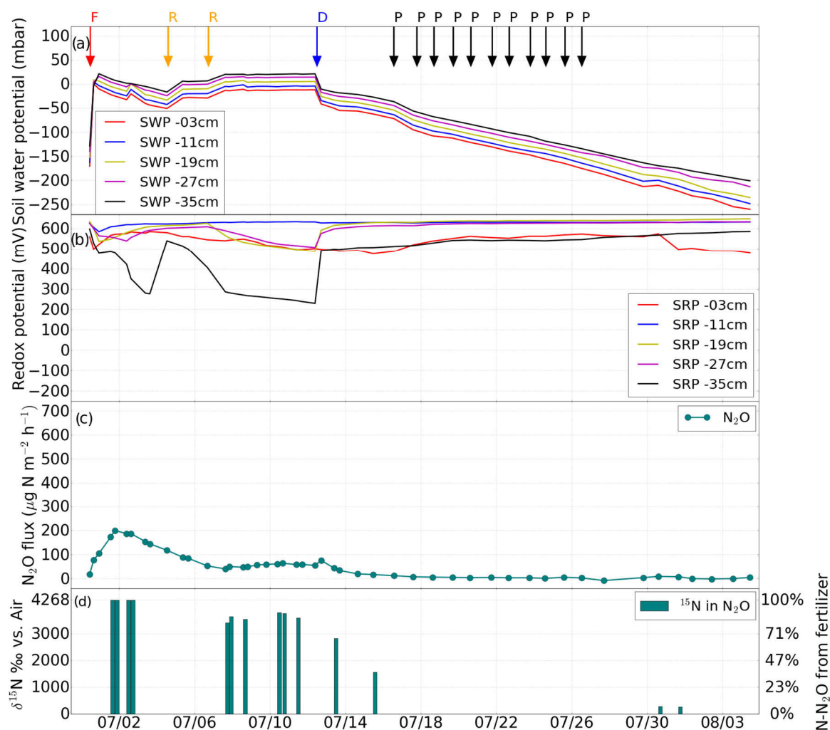
Figure 4. Experiment 3 (second fertilization). Changes in (a) soil water potential (SWP), (b) soil redox potential (SRP), (c) \text{N}_2\text{O} flux induced by drainage (D), irrigation with fertilizer (F), desaturation of the soil with pump (P), water table rise (R), (d) percentage of \text{N}_2\text{O} derived from the added fertilizer.
