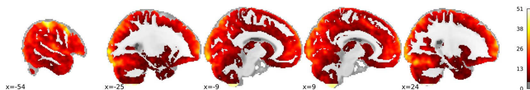
Fig. 3 Brain coverage of the IBC-dataset second-release. Group-level F-map, at a threshold of p < 0.05 , Bonferroni-corrected, representing the total area of the brain significantly covered by the tasks featuring solely the second release of the IBC dataset (FFX across tasks and subjects). One can easily observe an extensive brain coverage, with higher effects in lateral cortical areas by comparison with medial cortical areas and sub-cortical areas. We note that these results strictly follow the gray-matter structure, as an anatomically-defined gray-matter mask was used in the first-level GLM model (see Section “ Model Estimation ”).
