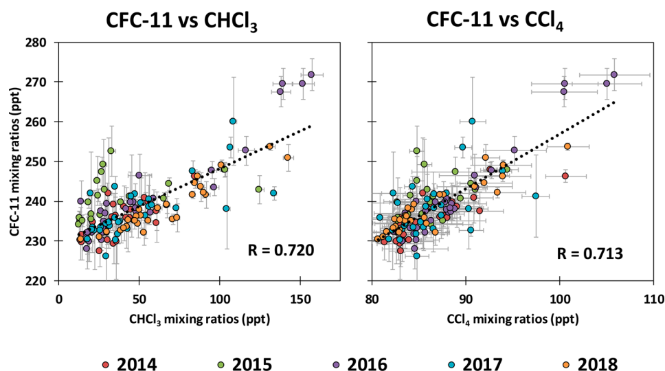
Figure 2. Interspecies correlations of CFC-11 mixing ratios with those of \text{CCl}_4 and \text{CHCl}_3 . For other interspecies correlations with CFC-11, see Figure S5. The dashed line is the trend line calculated by total least-squares regression using the York–Williamson method.
