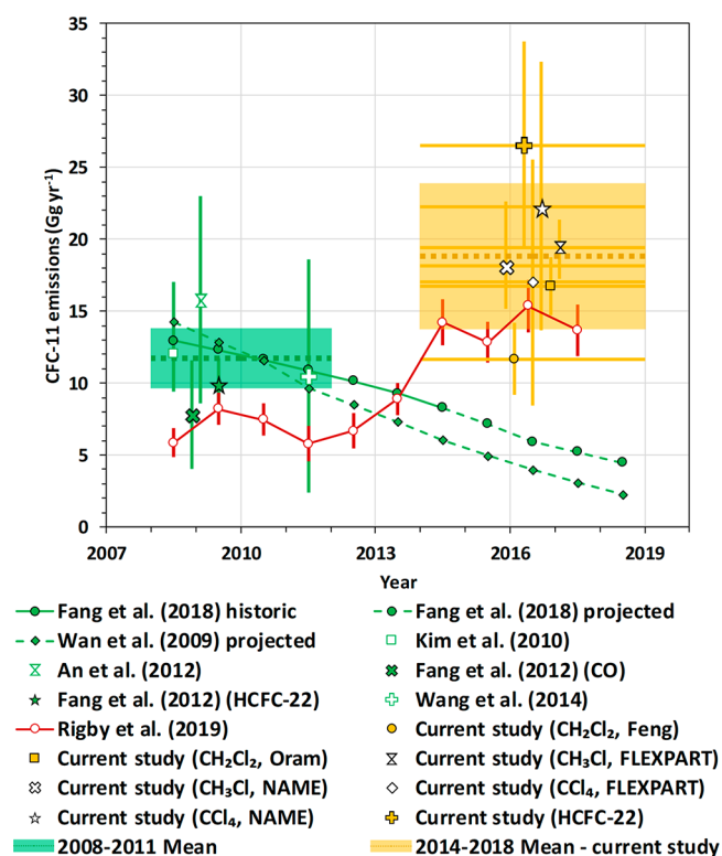
Figure 3. CFC-11 emissions in China and eastern China. 5,6,19,20,25–28 Data that cover means of several years have horizontal error bars to indicate the periods to which they relate. Vertical error bars show the uncertainties in the emission estimates. Data from the same years are offset slightly so that the error bars are visible. The data points joined by dashed lines are projections. The 2008–2011 mean is the mean of the estimates in Wan et al., 25 Kim et al., 26 An et al., 27 Fang et al., 19 Wang et al., 20 and Fang et al. 28 The 2014–2018 mean is the mean of the seven interspecies correlation estimates in this study. Emissions for the whole of China have filled data points, and emissions for eastern China have clear data points.
