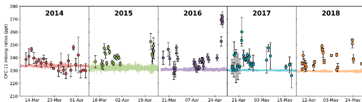
Figure 1. CFC-11 mixing ratios in Taiwan in 2014–2018. The measurement campaigns lasted for 1–3 months each year. Uncertainties represented by the error bars are described in the text. Hourly in situ measurements of CFC-11 mixing ratios at Mauna Loa, Hawaii, from the NOAA/ESRL Global Monitoring Division are included for comparison ( ftp://ftp.cmdl.noaa.gov/hats/cfcs/cfc11/insituGCs/CATS/hourly/ ). The standard deviation error bars of the Mauna Loa measurements are plotted in the same color as the data.
