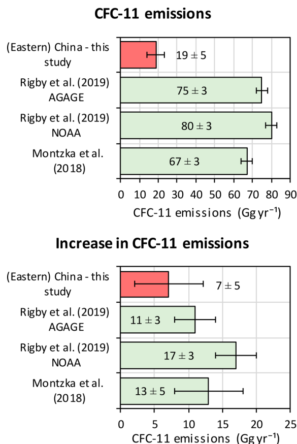
Figure 4. Global CFC-11 emissions (green bars) compared to the (eastern) China emissions in this study (red bar). Increase in global CFC-11 emissions (green bars) compared to the increase in (eastern) China emissions (red bar). These estimates are for slightly different time periods. The estimates from ref 5 are for 2014–2016 compared to 2002–2012. The estimates from ref 6 are for 2014–2017 compared to 2008–2012. This study's emission estimates are for 2014–2018 compared to 2008–2011.
