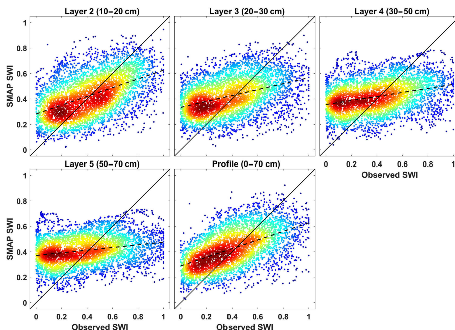
Figure 7. Comparisons of SMAP_L3 estimated–observed subsurface SWI for all stations during the growing seasons of 2015 to 2016. The smoothed color density in the scatter plot shows the density of points more clearly. The dash and solid lines are the best-fitted curve and “ y = x ” line, respectively.
