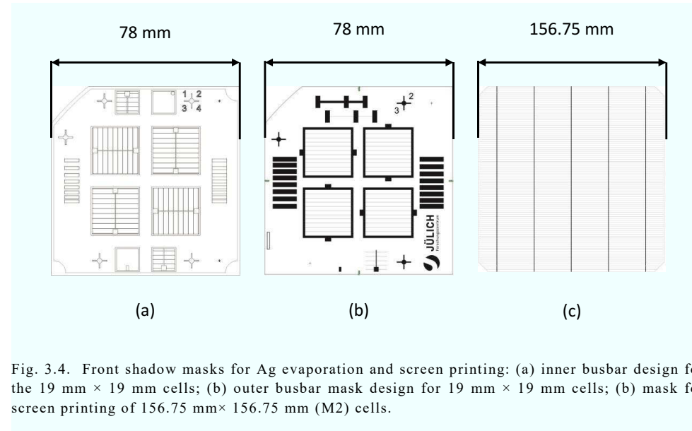
Fig. 3.4. Front shadow masks for Ag evaporation and screen printing: (a) inner busbar design for the 19 mm × 19 mm cells; (b) outer busbar mask design for 19 mm × 19 mm cells; (c) mask for screen printing of 156.75 mm × 156.75 mm (M2) cells.
