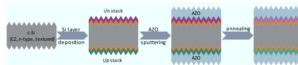
Fig. 6.14. Schematically illustration for the steps applied to the cell stack in the sequence of Si layer stacks deposition - AZO sputtering - annealing. Compared to the SHJ solar cells, the cell stack has the same structure, while with this sample, annealing was applied directly after the AZO sputtering and no further metallization.
