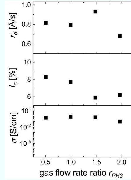
Fig. 4.4. Deposition rate, crystalline volume fraction, and conductivity variations of n-type nc-Si layers as a function of gas flow rate ratio r_{PH3} .
