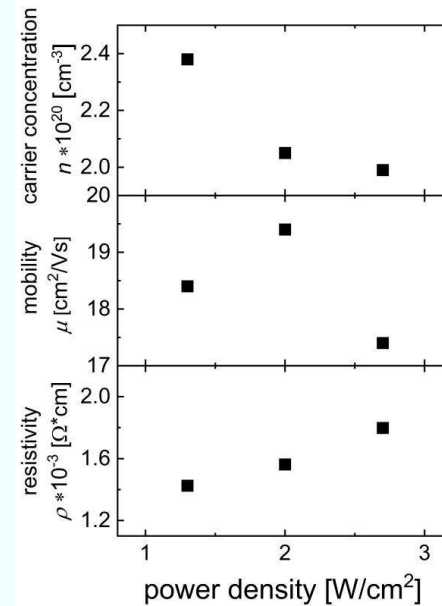
Fig. 4.14. Carrier concentration n , carrier mobility \mu , and resistivity \rho from Hall measurement for AZO films after annealing as a function of sputtering power densities of 1.3, 2.0 and 2.7 W/cm 2 , respectively.
