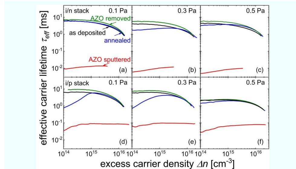
Fig. 6.4. Effective carrier lifetime versus excess carrier density curves for i/n (a)-(c) and i/p (d)-(f) symmetrical stacks with the treatment procedures: Si layer stack deposition - AZO sputtering - annealing - AZO removal. The experiments have been performed at room temperature with three AZO sputtering pressures: 0.1, 0.3, and 0.5 Pa as noted in each graph.
