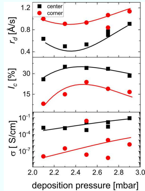
Fig. 4.8. Deposition rate, crystalline volume fraction, and conductivity variations of p-type nc-Si layers as a function of deposition pressure with TMB.
