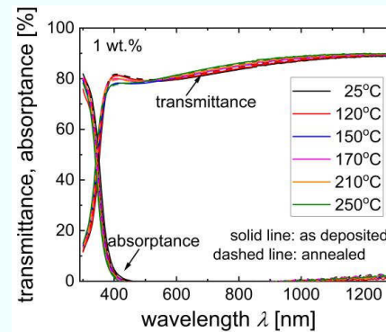
Fig. 4.15. Transmittance and absorptance spectra of AZO films as a function of sputtering heater temperature from 25°C to 250°C with 1 wt.% AZO target. The T/R is measured without considering the absorptance and reflectance of the glass substrate.
