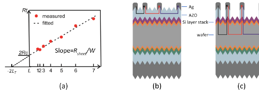
Fig. 3.6. Schematic illustration of (a) principle for the extracting of contact resistance from TLM measurement; (b) the assumed current flow route for the contact between AZO and silver; and (c) the assumed current flow route for the contact between AZO and silicon layers.
