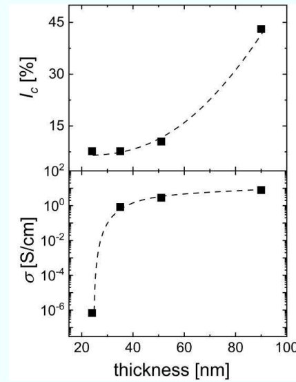
Fig. 4.6. Crystalline volume fraction and conductivity as a function of the thickness of n-type nc-Si layers deposited on intrinsic a-Si coated glass.
