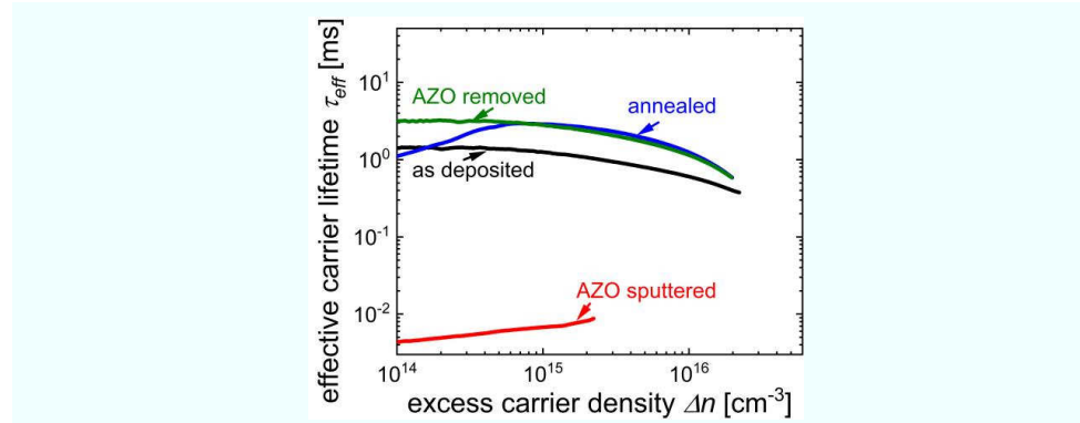
Fig. 6.19. Effective carrier lifetime versus excess carrier density curves for solar cell stack with full AZO coverage following the treatment procedure: Si layer stack deposition - AZO sputtering - AZO removal - annealing.
