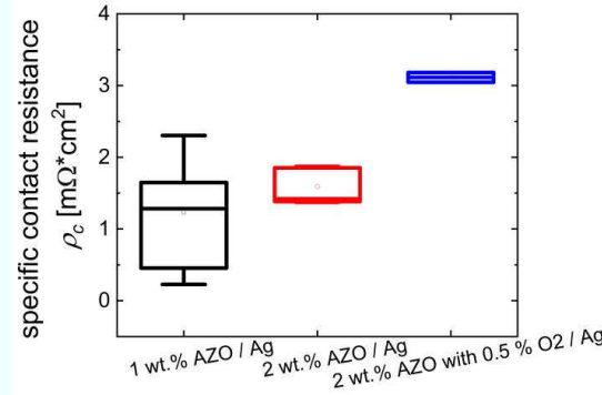
Fig. 5.20. Specific contact resistances at the interface between AZO and silver on n-type nc-Si growth surface for AZO sputtered with 1 wt.% target, 2 wt.% target, and 2 wt.% with oxygen in 19 \text{ mm} \times 19 \text{ mm} SHJ solar cells.
