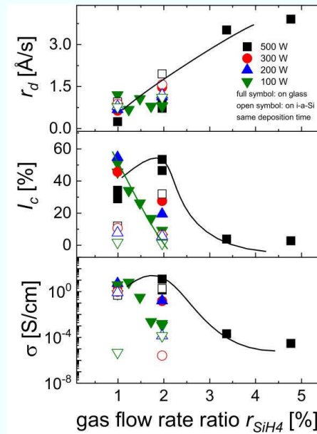
Fig. 4.2. Deposition rate, crystalline volume fraction, and conductivity of n-type nc-Si layers as a function of gas flow rate ratio r_{SiH_4} in the power range of 100 W to 500 W.
