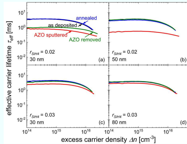
Fig. 6.12. Effective carrier lifetime versus excess carrier density curves for i/n symmetrical stacks deposited at the r_{SiH_4} of 0.02 with the thickness of 30 nm and 50 nm, and r_{SiH_4} of 0.03 with the thickness of 30 nm and 80 nm in the treatment procedures: Si layer stack deposition - AZO sputtering - annealing - AZO removal. The AZO was sputtered at RT with pressure of 0.1 Pa.
