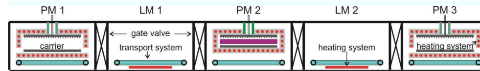
Fig. 3.2. Schematic illustration for the Si layer deposition system of AK 1000 large area in line PECVD system from Meyer Burger Company. The PM 2 is sketched with plasma-on status in the deposition.
