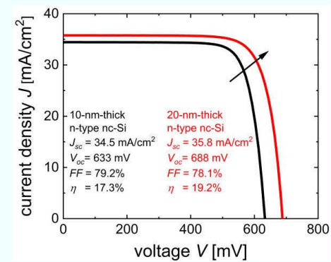
Fig. 5.6. Light current density-voltage curves of the SHJ solar cells with 10 nm- or 20 nm-thick n-type nc-Si, and p-type a-Si layers were used to form the junction at rear side of the cells. The photovoltaic parameters are indicated as inset.
