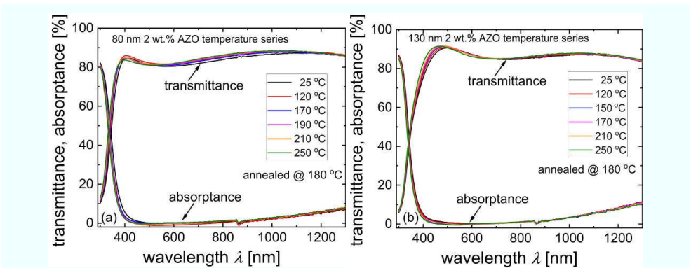
Fig. 4.22. Transmittance and absorbance spectra of AZO films as a function of sputtering heater temperature from 25°C to 250°C with the thickness of (a) 80 nm and (b) 130 nm.
