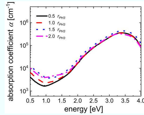
Fig. 4.5. Absorption coefficient as a function of energy for n-type nc-Si layers deposited with the gas flow rate ratio r_{PH3} in the range of 0.5-2.
