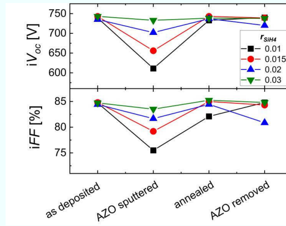
Fig. 6.11. Implied open circuit voltage and implied fill factor variations for i/n symmetrical stacks deposited with r_{SiH_4} of 0.01, 0.015, 0.02, and 0.03 with the treatment procedures: Si layer stack deposition - AZO sputtering - annealing - AZO removal. The AZO was sputtered at RT with pressure of 0.1 Pa. The n-type Si layers are deposited with same thickness.
