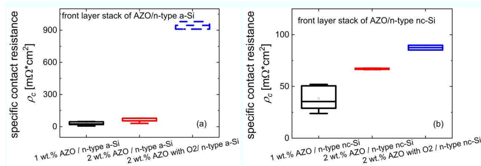
Fig. 5.21. Specific contact resistances for (a) front layer stack of AZO and n-type a-Si layers and (b) front layer stack of AZO and n-type nc-Si layers in 19 \text{ mm} \times 19 \text{ mm} SHJ solar cells.
