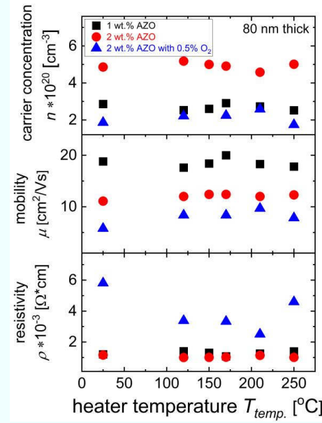
Fig. 4.21. Carrier concentration n , carrier mobility \mu , and resistivity \rho from Hall measurement for AZO films as a function of sputtering heater temperature from 25°C to 250°C with 1 wt.% target, 2 wt.% target, and 2 wt.% AZO target with 0.5% O 2 in the Argon precursor after annealing
