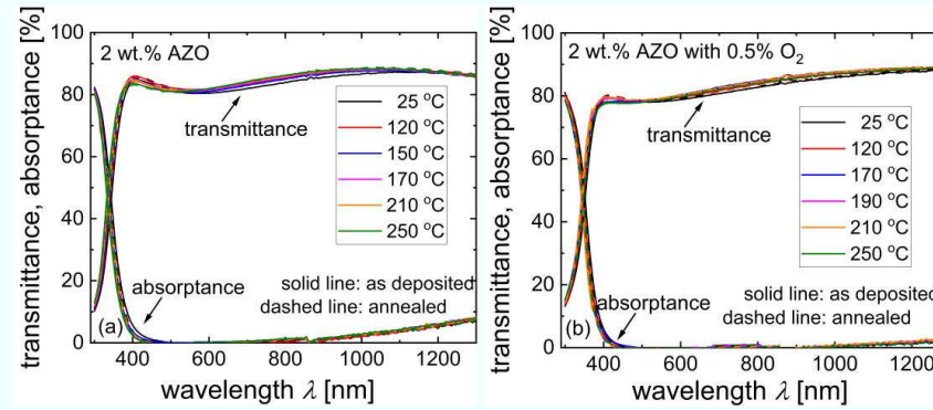
Fig. 4.17. Transmittance and absorbance spectra for AZO films as a function of sputtering heater temperature from 25°C to 250°C with (a) 2 wt.% AZO target and pure Argon precursor; (b) 2 wt.% AZO target and 0.5% O 2 in the Argon precursor.
