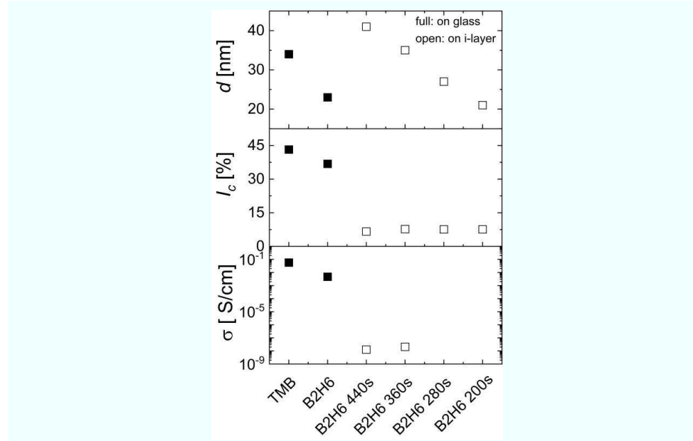
Fig. 4.9. Thickness, crystalline volume fraction, and conductivity variations of p-type nc-Si layers deposited with TMB or B 2 H 6 on glass, and with B 2 H 6 on intrinsic a-Si and varied deposition times of 440s, 360s, 280s, and 200s, respectively.
