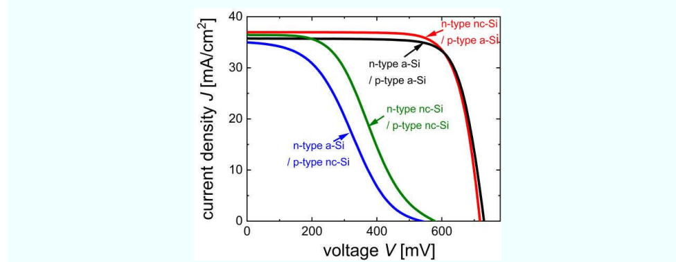
Fig. 5.3. Light current density-voltage curves of SHJ solar cells with the following four combinations of doped Si layers on the front and rear: (1) n-type a-Si / p-a-Si, (2) n-type nc-Si / p-type a-Si, (3) n-type a-Si / p-type nc-Si, and (4) n-type nc-Si / p-type nc-Si. Same RT sputtered AZO with 1 wt.% target was used as TCO in all presented cells.
