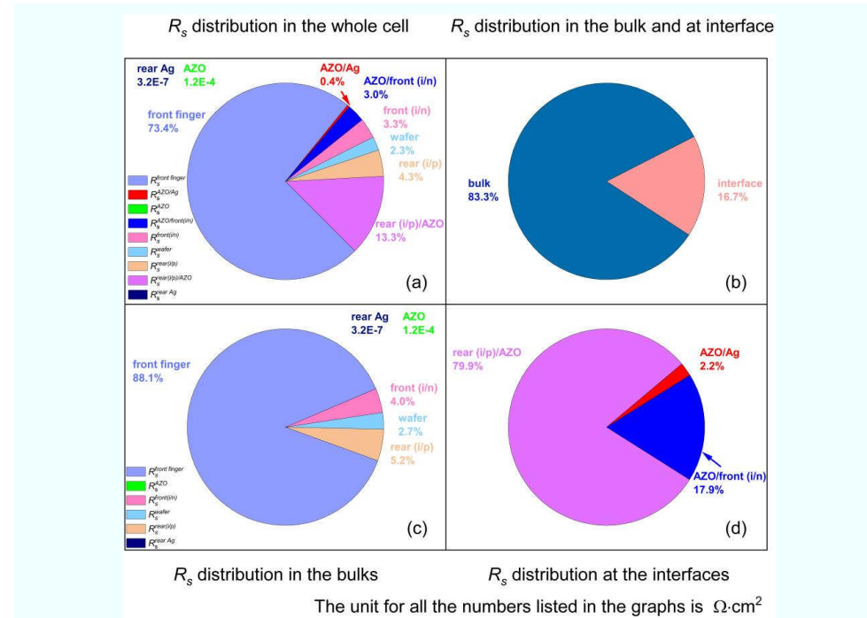
Fig. 8.8. Schematic illustration of the series resistance distribution in SHJ solar cells: (a) each series resistance component in solar cells; (b) series resistance distribution in the bulk and at the interface; (c) resistance distribution of each layer; (d) resistance distribution at the interface between layers.
