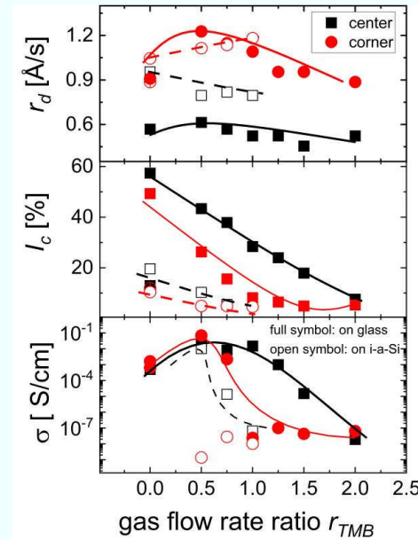
Fig. 4.7. Deposition rate, crystalline volume fraction, and conductivity variations of p-type nc-Si layers as a function of gas flow rate ratio r_{TMB} . Center and corner mean the sample position in deposition chamber.
