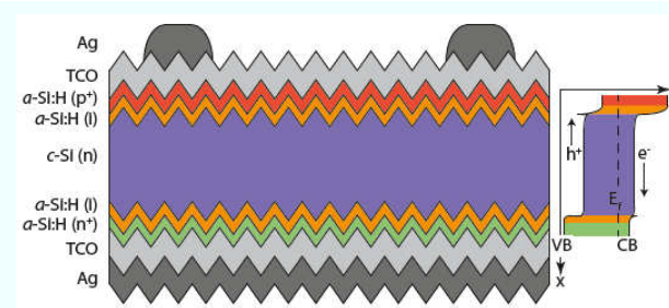
Fig. 2.3. Schematic cross-sections of the conventional silicon heterojunction solar cells [16].
