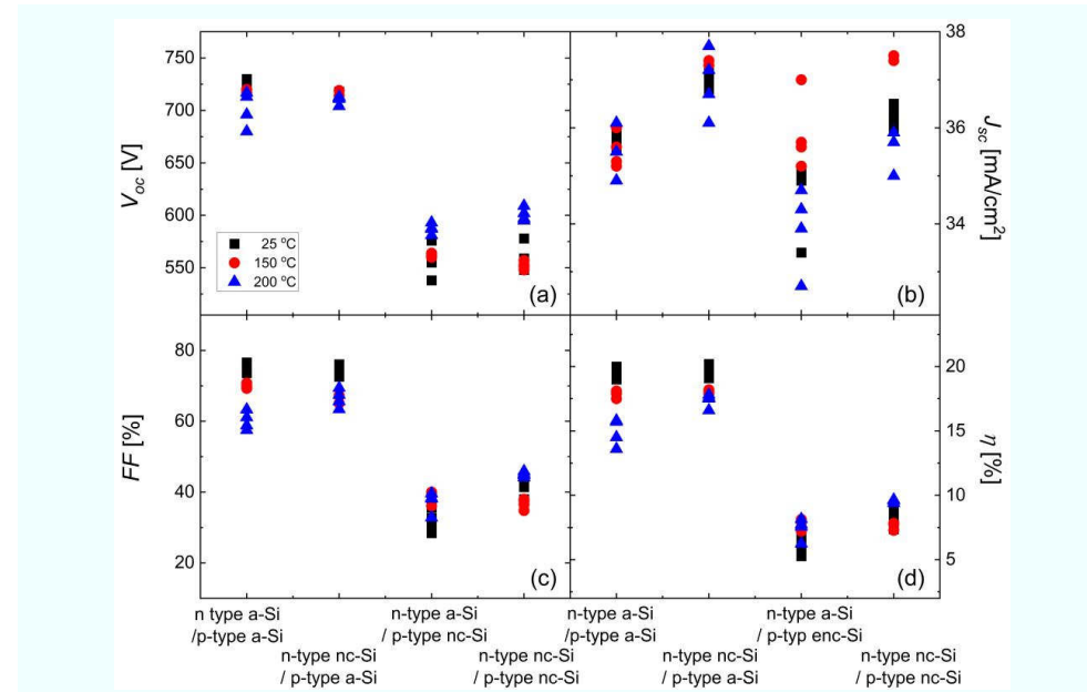
Fig. 5.12. Photovoltaic parameters of the SHJ solar cells with RT, 150°C, and 200°C sputtered 1 wt.% AZO and four combinations of silicon doped layers on the front and rear side: (1) n-type a-Si / p-type a-Si, (2) n-type nc-Si / p-type a-Si, (3) n-type a-Si / p-type nc-Si, and (4) n-type nc-Si / p-type nc-Si.
