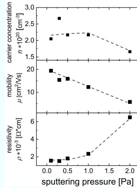
Fig. 4.12. Carrier concentration n , carrier mobility \mu , and resistivity \rho from Hall measurement of AZO films annealing as a function of sputtering pressure from 0.1 Pa to 2 Pa.
