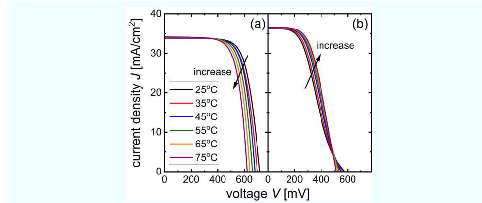
Fig. 7.3. Light J-V curves for the SHJ solar cells with (a) n-type a-Si and p-type a-Si; (b) n-type nc-Si and p-type nc-Si layer combinations measured at the temperatures of RT (25°C), 35°C, 45°C, 55°C, 65°C, and 75°C, respectively.
