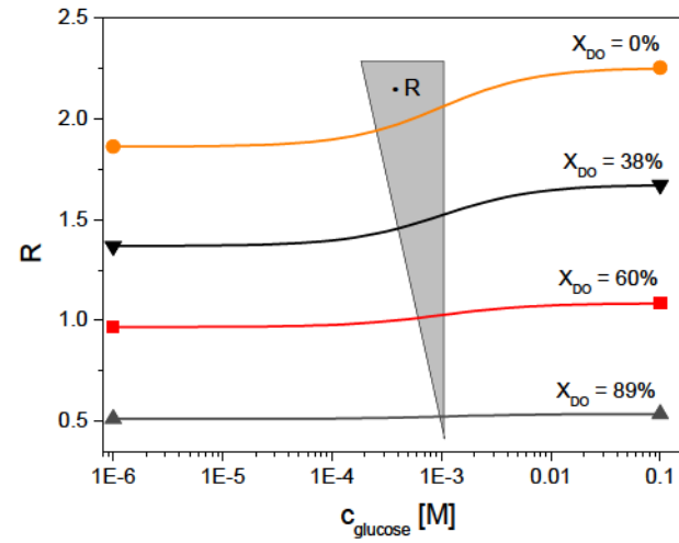
Figure 4.10: Effect of different donor-only fractions x_{D0} on ensemble read-out of glucose sensor construct no. 4. Donor-only fractions were determined with BTCCD (see Chap. 5). The sensor had an initial donor-only fraction of 38 % which was increased to 60 % and 89 % by photo-bleaching the acceptor with a 532 nm laser. Orange line shows hypothetical sensor signal for interpolation to vanishing donor-only fraction. Only R_{apo} and R_{max} were measured and connected to guide the eye according to Equation 4.2 with a fixed K_D . Adopted from [37].
