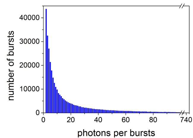
Figure B.4: Distribution of burst brightness of blue channel for dsDNA (Alexa488/Atto647N) reference. Adopted from [140] .
