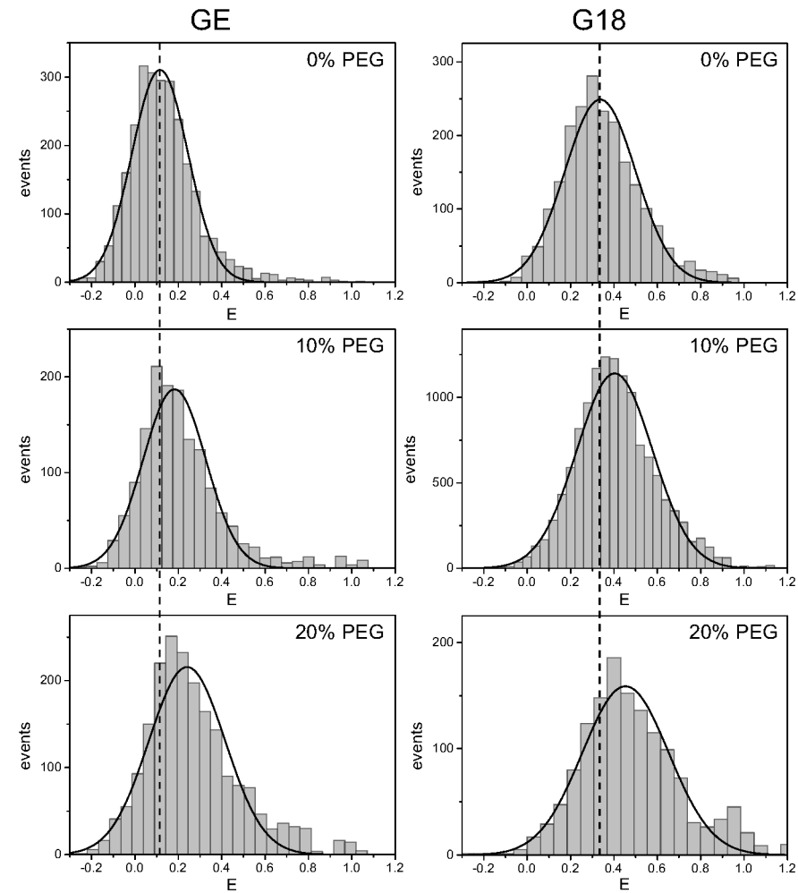
Figure 4.19: smFRET histograms of crowding sensor construct GE (left column) and G18 (right column) in absence of crowding (top row), for 10 w/w% PEG 6,000 (middle row), and for 20 w/w% PEG 6,000 (bottom row). All histograms are fitted with a single Gaussian distribution. The center of the non-crowded population is marked with a vertical dashed line to better notice the shift with increasing crowder concentrations. Adopted from [37].
