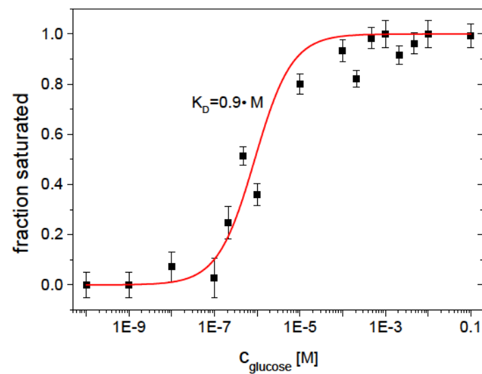
Figure 4.26: Fraction of glucose-saturated population in smFRET histogram of dye-labeled sensor as a function of glucose concentration. Isothermal binding curve is fitted in analogy to Equation 4.2 . Adopted from [13] .
