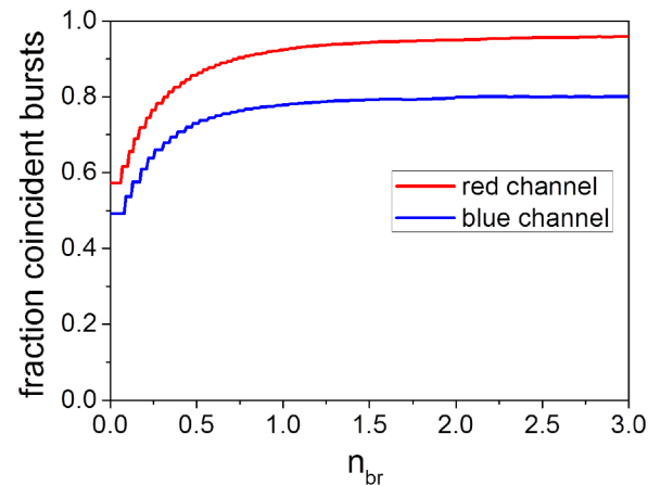
Figure 5.13: Coincidence fractions of dsDNA (Alexa 488/Alexa 647) reference as a function of brightness threshold. Adopted from [140].
