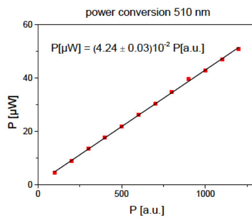
Figure A.4: Conversion of power readings obtained by power diode ( a.u. ) to real power ( \mu W ). Power was measured at the objective position using a power meter.
