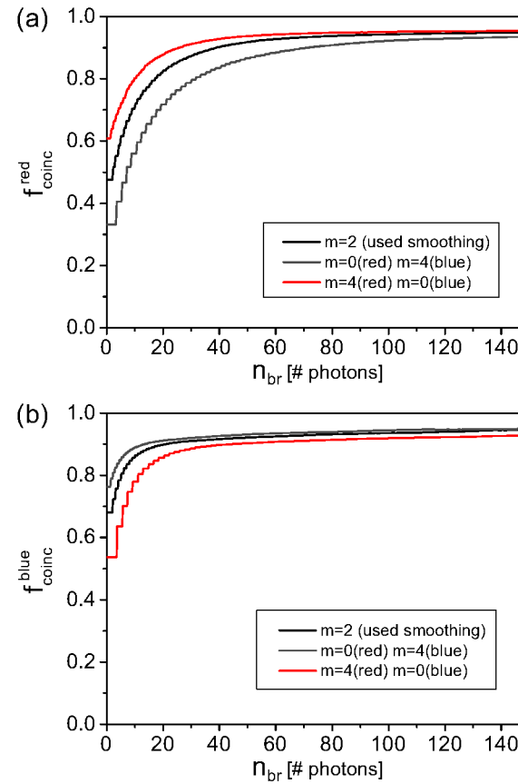
Figure 5.16: Fraction of coincident (a) red and (b) blue bursts as a function of brightness threshold for dsDNA reference (Alexa 488/Atto 647N). The TPL time trace smoothing parameter m is varied from the used value (black lines) conversely for both channels. The red and blue coincidence fractions show an opposite dependency on the smoothing value combinations because a higher smoothing value leads to a preselection of bright bursts in the respective channel and, hence, to higher coincidence fractions and a saturation at smaller brightness thresholds. Adopted from [140] .
