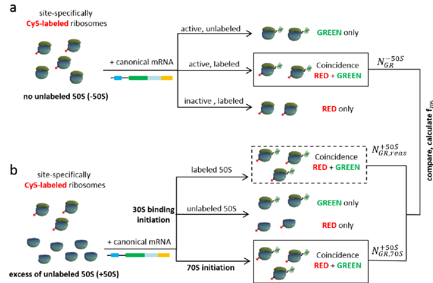
Figure 5.28: Concept of initiation investigation. Adopted from [140].
