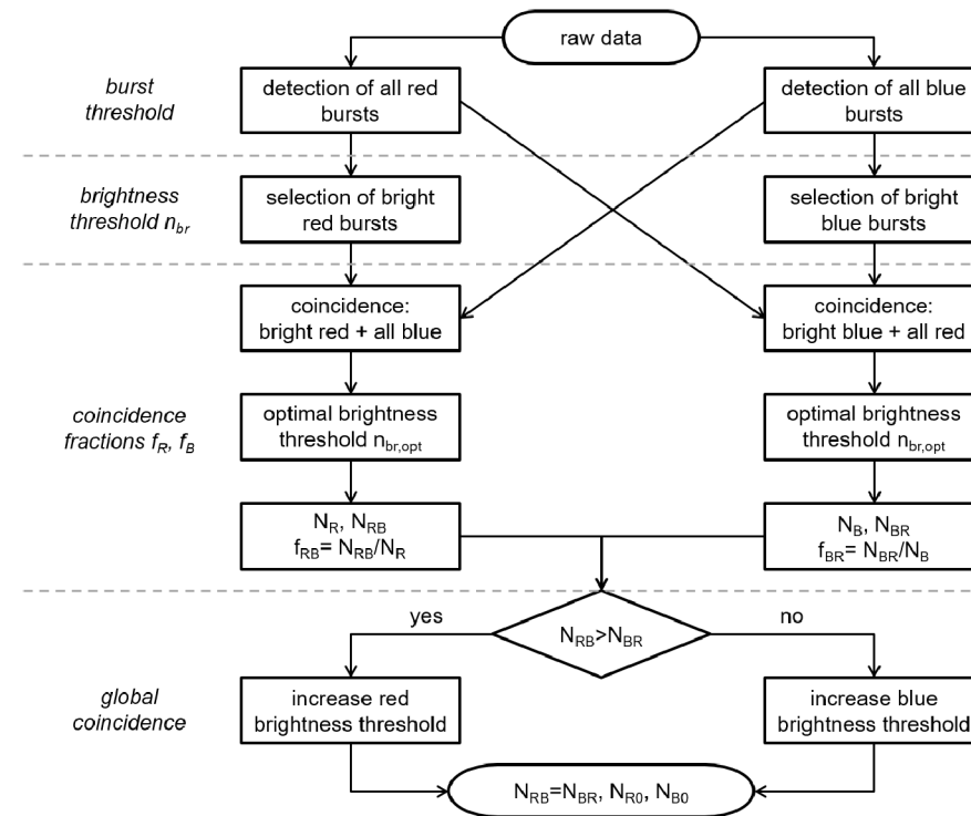
Figure 5.5: Workflow of brightness-gated two-color coincidence detection. Adopted from [140].
