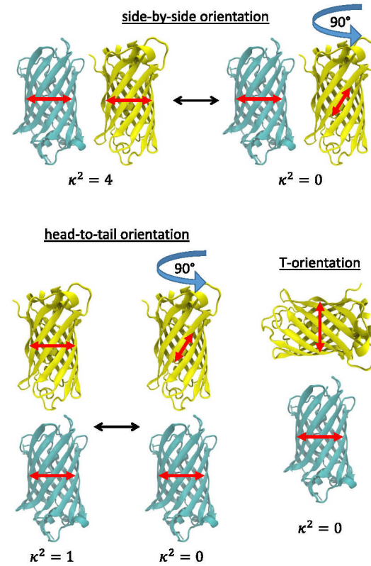
Figure 4.2: Possible spatial arrangements of two fluorescent proteins (pdb entries: 3ztf (CFP), 1myw (YFP)) and respective range of orientation factor \kappa^2 . Dipole moments are depicted as red arrows.
