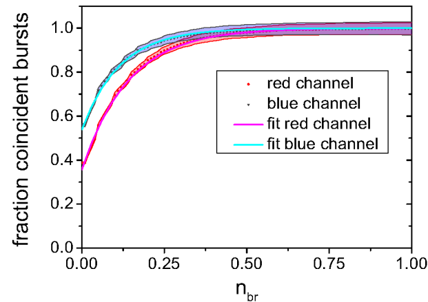
Figure 5.8: Fitting of coincidence fractions of nano-bead reference.
