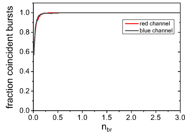
Figure 5.10: Coincidence fractions of TetraSpeck beads as a function of brightness threshold. After a steep increase for low thresholds both colors show full coincidence.
