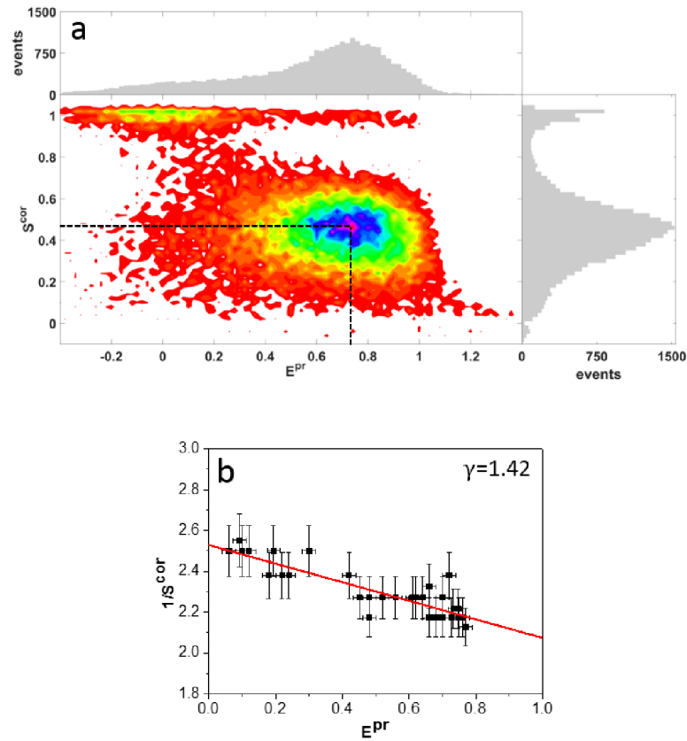
Figure 4.15: (a) 2D-plot of proximity ratio E^{pr} and corrected stoichiometry S^{cor} is used to identify center of donor-acceptor population (dashed lines). (b) Plot of 1/S^{cor} against E^{pr} for all investigated glucose sensor constructs. Linear fit (red line) is used to calculate \gamma (see Eq 4.14). Adopted from [37].
