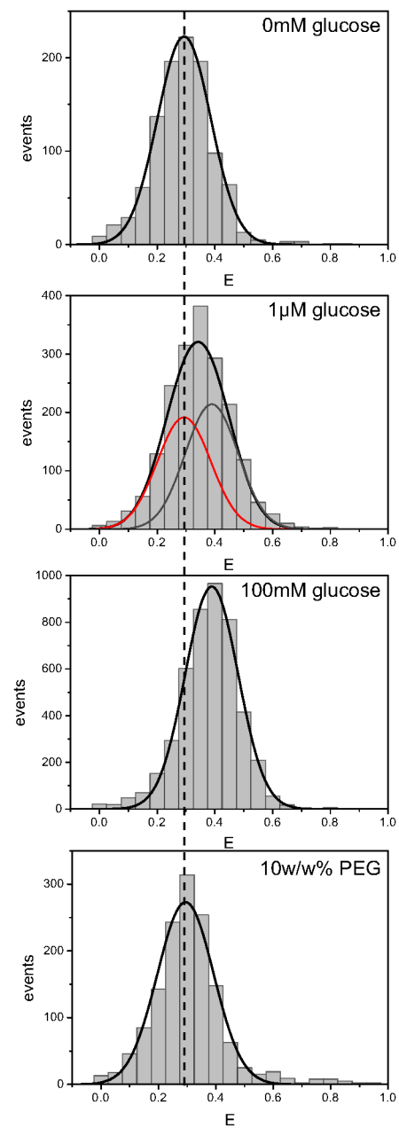
Figure 4.25: smFRET histogram of dye-labeled glucose sensor in absence of glucose, at glucose concentration equal to K_D ( 1\ \mu\text{M} ), at saturating glucose concentration of 100\ \text{mM} , and for 10\ \text{w/w\%} PEG 6,000. Adopted from [13].
