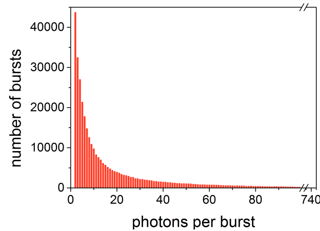
Figure 5.11: Distribution of burst brightness of red channel for dsDNA (Alexa 488/Atto 647N) reference. Distribution of blue channel looks similar and can be found in Appendix Figure B.4. Adopted from [140].
