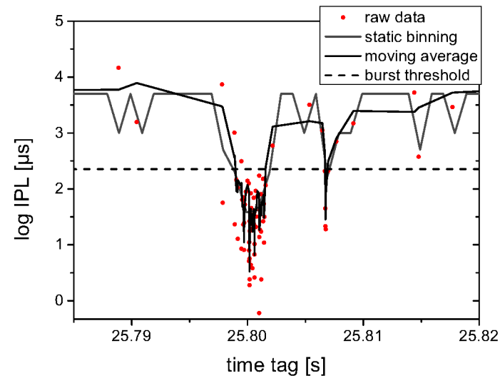
Figure 3.12: Exemplary IPL time trace with static binning and using a moving average filter. Long bursts are identified similar with both methods but static binning starts to become imprecise for dim bursts.
