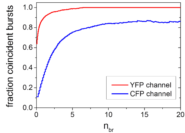
Figure 5.23: Coincidence fractions of crowding sensor GE as a function of brightness threshold. Adopted from [140].
