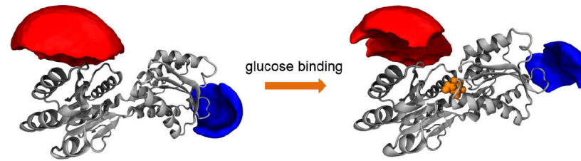
Figure 4.24: Visualization of donor (blue) and acceptor (red) AV clouds in open (left) and closed (right) conformation of MglB. Adopted from [13].
