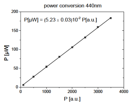
Figure A.3: Conversion of power readings obtained by power diode ( a.u. ) to real power ( \mu W ). Power was measured at the objective position using a power meter.
