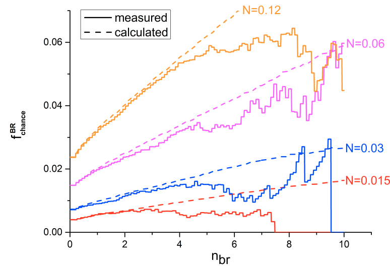
Figure 5.20: Chance coincidences of freely-diffusing Alexa 488 (B) and Alexa 647 (R) dyes. Concentration of dyes is adjusted to achieve same number of molecules in red and blue detection volume ( N_R = N_B = N/2 ). BTCCD analysis (solid line) is compared to predicted fraction of blue chance coincidence according to Equation 5.18
