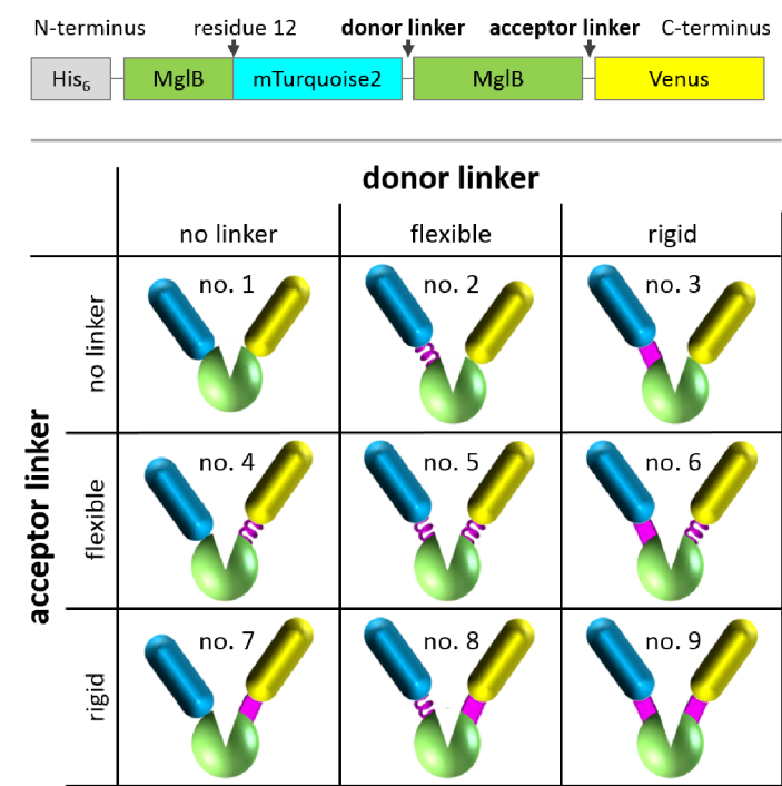
Figure 4.3: upper panel: Composition of the glucose sensor. The N-terminus begins with a polyhistidine followed by the glucose binding protein (MglB). The donor (mTurquoise2) is internally fused after residue 12 followed by the donor linker, the rest of MglB, the acceptor linker and the acceptor (Venus) itself. lower panel: Combination of three different linkers for donor or acceptor position results in 9 different sensor constructs. Adopted from [37].
