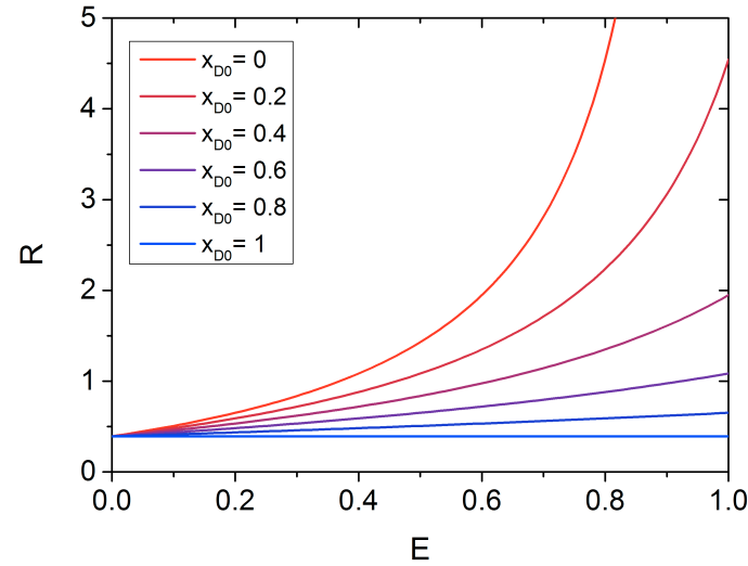
Figure 4.9: Conversion of transfer efficiency E to peak intensity ratio R for various donor-only fractions according to Equation 4.3. Donor and acceptor are mTurquoise2 and Venus, respectively. Quantum yields were determined as \Phi_D = 0.90 and \Phi_A = 0.59 which results in c_D^D = 0.0139 , c_D^A = 0.00546 , and c_A^A = 0.0144 . Adopted from [37].
