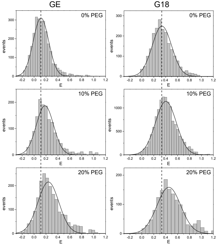
Figure 4.19: smFRET histograms of crowding sensor construct GE (left column) and G18 (right column) in absence of crowding (top row), for 10 w/w% PEG 6,00 (middle row), and for 20 w/w% PEG 6,000 (bottom row). All histograms are fitted with a single Gaussian distribution. The center of the non-crowded population is marked with a vertical dashed line to better notice the shift with increasing crowder concentrations. Adopted from [37].
