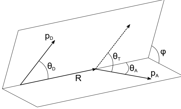
Figure 3.4: Orientational dependency of FRET.
