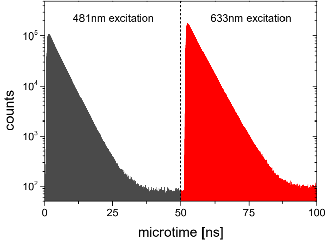
Figure 3.9: Principle of pulsed interleaved excitation (PIE).
