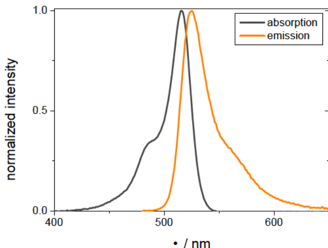
Figure 3.2: Absorption and fluorescence emission spectra of yellow fluorescent protein variant Venus.
