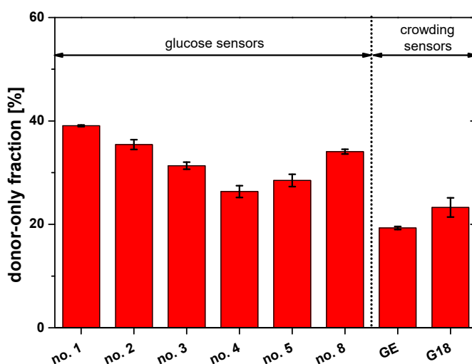
Figure 5.24: Donor-only fractions of FRET-based biosensors. Adopted from [37].
