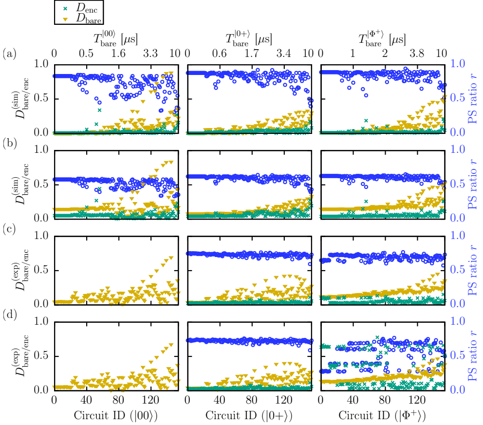
Figure 7.8: Test of the fault-tolerant protocol using (a) the transmon simulation model defined in Section 3.4.5; (b) the same model with an additional measurement error of \epsilon = 0.08 (cf. Eq. (7.19)); (c) the ibmqx5 [IBM2018a] on April 19, 2018; (d) the ibmqx5 on April 20, 2018. Shown are the statistical distances D_{\text{bare}} for the bare circuits (yellow triangles) and D_{\text{enc}} for the encoded circuits (green crosses) as defined in Eq. (7.18), as well as the corresponding postselection ratios r (blue circles). The three panels in each row correspond to the three initial states in Tab. 7.3 (the left panels in (c) and (d) only contain data for the bare circuits because the encoded circuits for the initial state |00\rangle cannot be run on the ibmqx5 ). The circuit IDs on the bottom axis are defined in Listing 7.1. They are sorted by the total time T_{\text{bare}}^{(00)} required to simulate all pulses of the bare circuits for the initial state |00\rangle (some representative time scales are indicated on the top axis).
