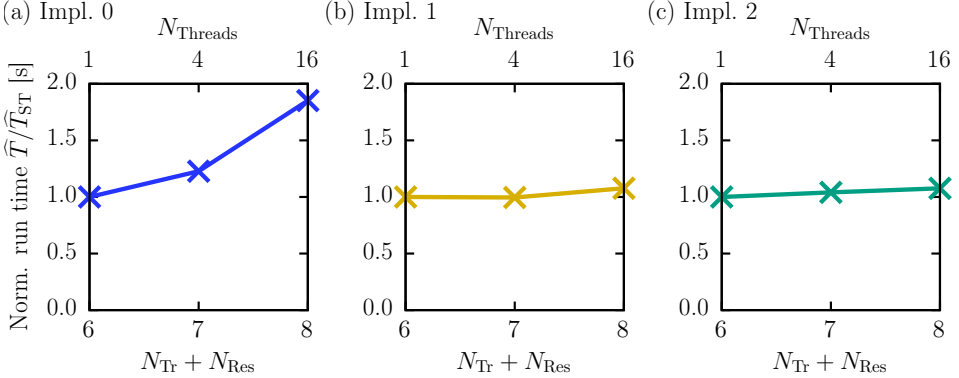
Figure 4.4: Weak scaling performance of the normalized run time \hat{T}/\hat{T}_{\text{ST}} using (a) implementation 0 where \hat{T}_{\text{ST}} = 1.202 \text{ s}/6 , (b) implementation 1 where \hat{T}_{\text{ST}} = 1.188 \text{ s}/6 , (c) implementation 2 where \hat{T}_{\text{ST}} = 1.188 \text{ s}/6 . Lines are drawn to guide the eye.
