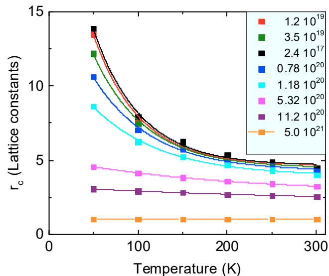
Figure 5. Spatial extent of polar nano-regions as a function of temperature and various carrier concentrations n as indicated in the inset to the figure.
