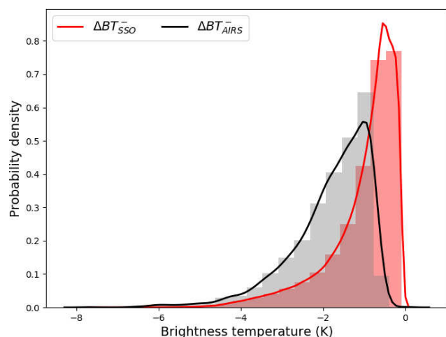
Figure 2. Comparison of the probability distribution of brightness temperature perturbations (K) due to mountain-wave-induced stratospheric cooling over the Antarctic Peninsula between the parameterisation scheme \Delta BT_{SSO}^- (red line) and the AIRS observations \Delta BT_{AIRS}^- (black line) for May to October. The AIRS values are from the 666.5\text{ cm}^{-1} radiance channel, for a 16-year period from 2002 to 2017 (and includes some contribution from non-orographic wave sources). The parameterised values are the weighted sum of \Delta T_{SSO}^- from the perturbation run over all vertical model levels from 15 to 45 km (using the AIRS kernel function for the 666.5\text{ cm}^{-1} radiance channel), which is required to convert \Delta T_{SSO}^- to \Delta BT_{SSO}^- . Note that a minimum threshold of BT < -0.1\text{ K} is used to reduce the inclusion of noise and spurious events. Both the parameterised and AIRS results are computed within the box indicated in Fig. 1.
