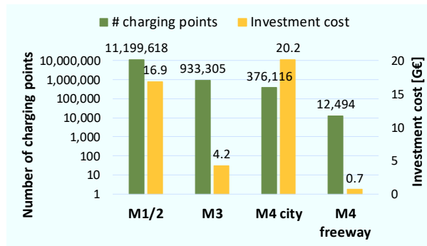
Figure 8 – Number of PEV charging points and related investment cost, in case B.
