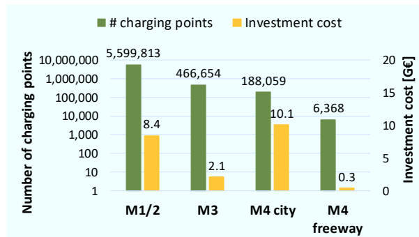
Figure 13 – Number of PEV charging points and related investment cost, in case C.
