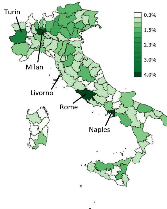
Figure 3 – Relative distribution of ZEVs and subsequent energy vector demand expected in 2050, by province.
