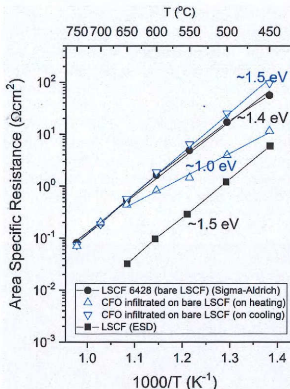
Figure 4 Arrhenius plot of ASR of total polarization losses of symmetrical LSCF
