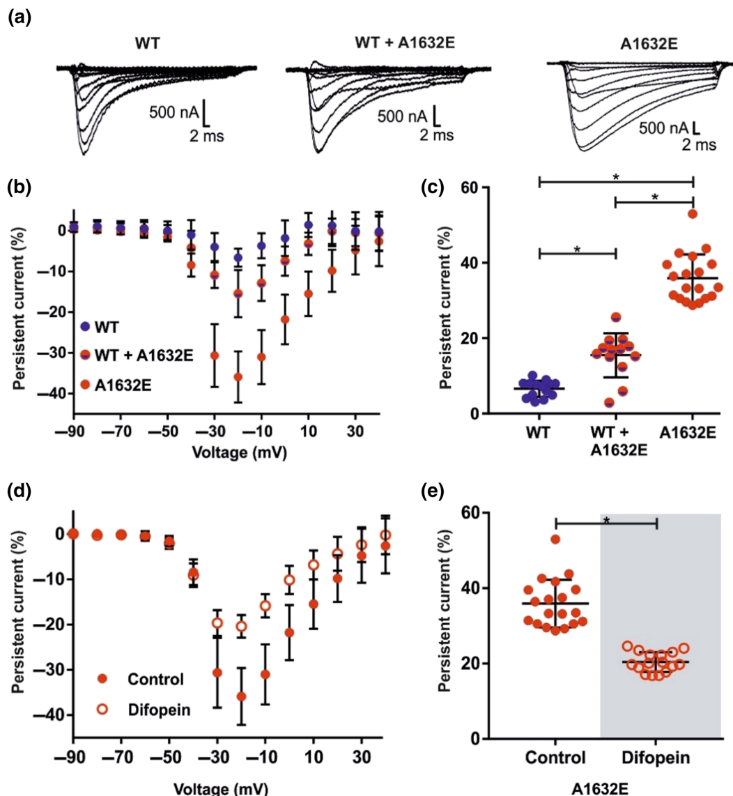
FIGURE 7 Expression of hNav1.7/WT and hNav1.7/A1632E channels in Xenopus laevis oocytes. (a) Representative current traces of X. laevis oocytes expressing hNav1.7/WT (left panel), hNav1.7/A1632E (right panel) or the combination of WT and A1632E (middle panel) elicited by stepwise depolarizations from -90 mV to +40 mV in 10 mV increments (from a holding potential of -100 mV). (b) Relative persistent current of oocytes expressing the indicated hNav1.7 channels. The measured persistent current at each voltage step was normalized to the maximum peak inward current of each oocyte. Oocytes were injected with the following amounts of cRNA(s) encoding the indicated Na v -channel: hNav1.7/WT: 30 ng; hNav1.7/A1632E: 30 ng; hNav1.7/WT + hNav1.7/A1632E: 60 ng (30 ng each). (c) Maximal relative persistent current of each cell is shown as it was used for statistical comparison. Data shown are individual values with means \pm SD; hNav1.7/WT, N = 14 ; hNav1.7/WT + hNav1.7/A1632E, N = 13 ; hNav1.7/A1632E, N = 19 . Difference of means: hNav1.7/WT - hNav1.7/WT + hNav1.7/A1632E: -8.8%, 95% CI of difference of means [-13.9; -3.8]; hNav1.7/WT - hNav1.7/A1632E: -29.3 [-33.9; -24.7]; hNav1.7/WT + hNav1.7/A1632E - hNav1.7/A1632E: -20.5 [-25.2; -15.7]. * P < 0.05 , significantly different as indicated. (d) Relative persistent current of oocytes expressing the hNav1.7/A1632E channel in absence or presence of difopein. The measured persistent current at each voltage step was normalized to the maximum peak inward current of each oocyte. Oocytes were injected with the following amounts of cRNA(s) encoding either the hNav1.7/A1632E channel or the hNav1.7/A1632E channel + difopein: hNav1.7/A1632E: 30 ng; hNav1.7/A1632E + difopein: hNav1.7/A1632E 30 ng + difopein 12 ng. (e) Maximal relative persistent current of each cell is shown as it was used for statistical comparison. Data shown are individual values with means \pm SD; hNav1.7/A1632E, N = 19 ; hNav1.7/A1632E + difopein, N = 16 . Analyzed using a Mann-Whitney test. Difference between medians: -13.6%, 95% CI of difference of means: [-18.5; -11.4]. For exact numbers of mean, SD, and N of each data point (b, d), please refer to Tables S10-S14 * P < 0.05 , significantly different as indicated
