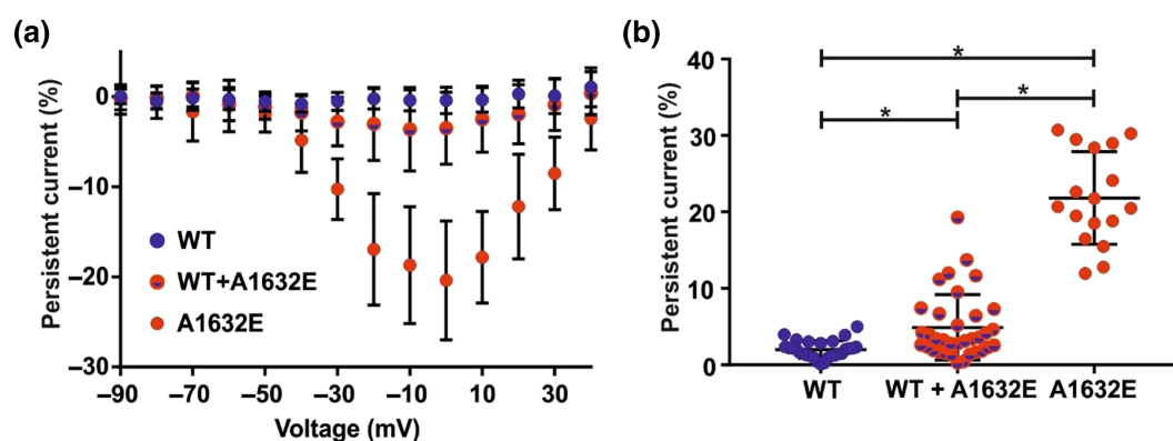
FIGURE 3 Co-expression of hNa v 1.7/WT and hNa v 1.7/A1632E in a Na v 1.7 stable cell line disproportionally affects persistent current. (a) Relative persistent current of HEK cells expressing the indicated hNa v 1.7 channels. The measured persistent current at each voltage step was normalized to the peak inward current of the cell. Concentration of transfected cDNA: WT: Na v 1.7 stable cell line; WT + A1632E: 1.25 μg hNa v 1.7/A1632E + 0.25 μg GFP (Na v 1.7 stable cell line); A1632E: 1.25 μg hNa v 1.7/A1632E + 0.25 μg GFP (HEK293T cells). Data were not statistically analysed. For mean, SD, and N of each data point, please refer to Tables S5–S7. (b) Maximal relative persistent of each cell as used for statistical analysis. Data shown are individual values with means ± SD; hNa v 1.7/WT, N = 28; hNa v 1.7/WT + hNa v 1.7/A1632E, N = 35; hNa v 1.7/A1632E, N = 17. Difference of means: hNa v 1.7/WT – hNa v 1.7/WT + hNa v 1.7/A1632E: –2.9%, 95% CI of difference of means: [–5.4; –0.4]; hNa v 1.7/WT – hNa v 1.7/A1632E: –19.8% [–22.9; –16.8]; hNa v 1.7/WT + hNa v 1.7/A1632E – hNa v 1.7/A1632E: –16.9% [–19.8; –14.0]. *P < 0.05, significantly different as indicated
