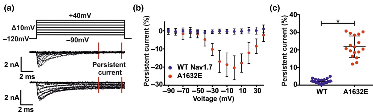
FIGURE 1 Expression of hNav1.7/A1632E channels causes a prominent persistent current compared to that in a Nav1.7 channel stable cell line. (a) Representative traces of hNav1.7/WT (middle panel) and hNav1.7/A1632E (bottom panel) sodium currents. The persistent current was measured in the indicated range (between the red bars). The voltage protocol is shown in the top panel. Concentration of transfected cDNA: WT: Nav1.7 stable cell line; A1632E: 1.25 µg hNav1.7/A1632E + 0.25 µg GFP (HEK293T cells). (b) Relative persistent current of HEK cells expressing the indicated hNav1.7 channels. The measured persistent current at each voltage step was normalized to the peak inward current of the cell. Data were not statistically analysed. For means, SD, and N for each data point, please refer to Tables S3–S4. (c) Maximal relative persistent current of each cell as used for statistical comparison. Data shown are individual values with means \pm SD; hNav1.7/WT, N = 28; hNav1.7/A1632E, N = 17. Difference of means: 19.8%, 95% CI of difference of means: [17.5; 22.2]. * P < 0.05 , significantly different as indicated
