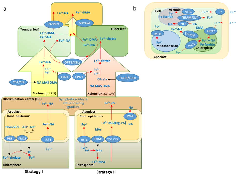
Fig. I-1: a) Scheme of Fe uptake from rhizosphere (Strategy I, Strategy II) and translocation in plant. b) Scheme of Fe translocation in plant cell. Red arrows indicate the dominant Fe pathways and transfers between different Fe pools (different colors), with blue ellipses indicating specific transporters which adjust Fe loading and unloading from plasma membrane.
