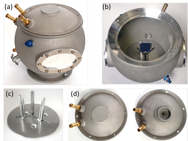
FIG. 2. (a) Photograph of the 3D printed sample chamber with connectors and aluminum foil windows. The golden hose nipples are connectors to the heating circuit, and the blue compression fittings can be used as in- and outlet for a gas flow. The flange nipple on the bottom left is used to connect to the electronics inside the chamber via a LEMO plug. (b) Interior view of the chamber where the sample holder and sample (blue square) are located. (c) Close-up view of the sample holder. (d) Top view showing the standard lid (left) and a lid with a calcium fluoride ( \text{CaF}_2 ) glass for complementary spectral reflectance measurements (right).
