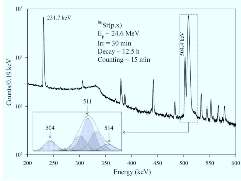
FIG. 4: A partial HPGe \gamma -ray spectrum in transient equilibrium of ^{85}\text{Sr}^{\text{m}} (1.127 h) with ^{85}\text{Y}^{\text{g}} (2.68 h), their corresponding 232- and 504-keV \gamma rays are labeled. Inset represents fitted peaks by Fitzpeak gamma analysis software in selected region. 504 keV \gamma peak separated neatly from the 511 keV annihilation peak. The 514 keV \gamma peak comes from ^{85}\text{Sr} (64.849 d) decay. The annihilation peak was fitted with three component peaks, 511 (labeled) and two others by the sides, owing to its characteristic broader width compared to other \gamma -ray peaks, used for FWHM calibration.
