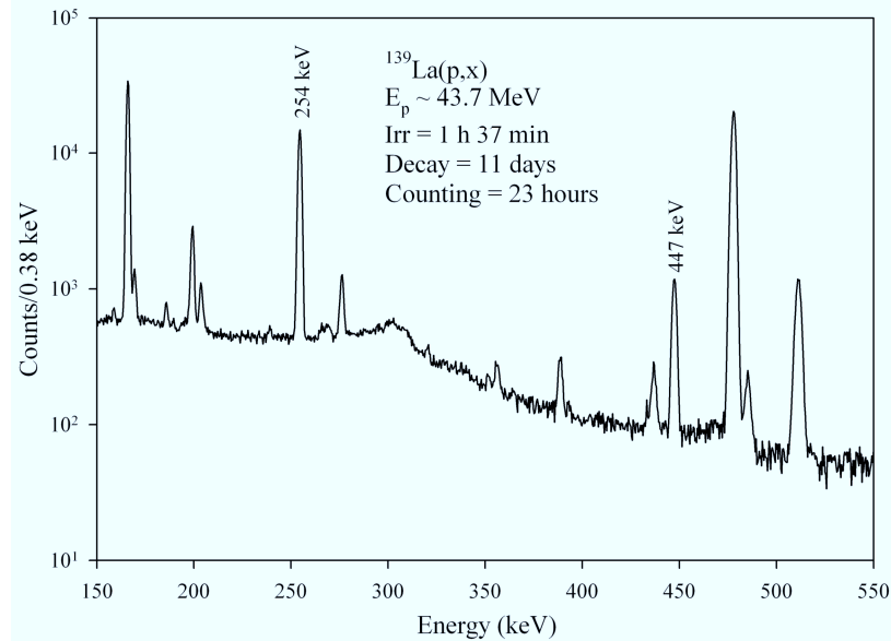
FIG. 2: A partial HPGe \gamma -ray spectrum of ^{137}\text{Ce}^{\text{g}} (9 h) in transient equilibrium with ^{137}\text{Ce}^{\text{m}} (34.4 h), their corresponding 447- and 254-keV \gamma rays are labeled.
