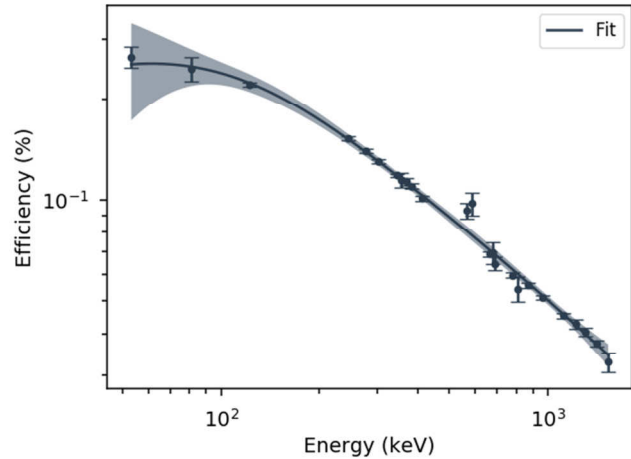
FIG. 3: The measured HPGe detector efficiency at 30 cm (points with uncertainty) along with the fitted line. The shaded region represents the 1\sigma confidence band.
