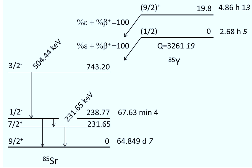
FIG. 5: Partial ^{85}\text{Sr} level scheme (not in scale) from ^{85}\text{Y}^g (2.68 h) and ^{85}\text{Y}^m (4.86 h) decays [38], showing 504- and 232-keV \gamma rays from the 743- and 232-keV levels, respectively.
