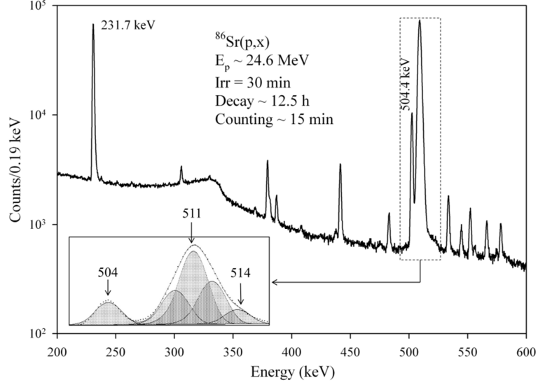
FIG. 4: A partial HPGe \gamma -ray spectrum in transient equilibrium of ^{85}\text{Sr}^{\text{m}} (1.127 h) with ^{85}\text{Y}^{\text{g}} (2.68 h), their corresponding 232- and 504-keV \gamma rays are labeled. Inset represents fitted peaks by Fitzpeak gamma analysis software in selected region. 504 keV \gamma peak separated neatly from the 511 keV annihilation peak. The 514 keV \gamma peak comes from ^{85}\text{Sr} (64.849 d) decay. The annihilation peak was fitted with three component peaks, 511 (labeled) and two others by the sides, owing to its characteristic broader width compared to other \gamma -ray peaks, used for FWHM calibration.
