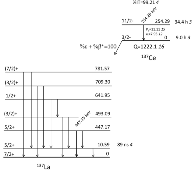
FIG. 1: Partial level scheme (not in scale) showing 254- and 447-keV \gamma rays from the ^{137}\text{Ce}^{\text{m}} (34.4 h) isomeric decay and the ^{137}\text{Ce}^{\text{g}} (9.0 h) decay, respectively. Detailed decay schemes can be found in Ref. [14]. \%P_\gamma(254) and conversion coefficient, \alpha , are also listed.
