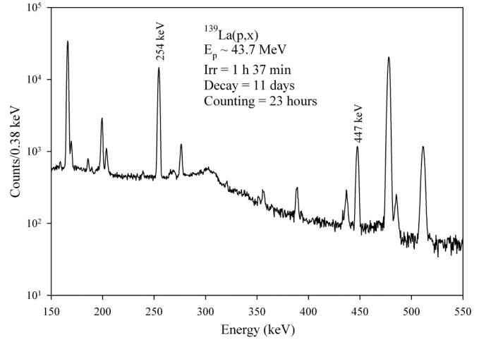
FIG. 3. A partial HPGe \gamma -ray spectrum of ^{137}\text{Ce}^g (9 h) in transient equilibrium with ^{137}\text{Ce}^m (34.4 h); their corresponding 447- and 254-keV \gamma rays are labeled.
