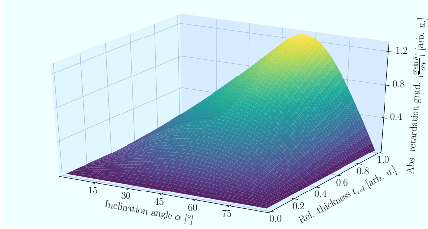
FIGURE 4.4: Absolute retardation gradient with respect to inclination \left| \frac{\partial \sin \delta}{\partial \alpha} \right| as a function of inclination and relative thickness t_{\text{rel}} .
