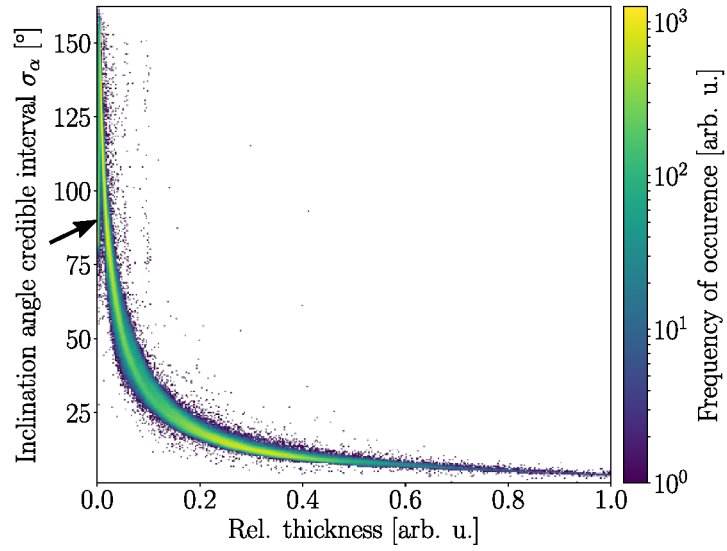
FIGURE 6.12: Correlation of relative thickness t_{\text{rel}} and inclination angle credible interval \sigma_\alpha . The plot displays a two-dimensional histogram of the relative thickness and inclination angle credible interval maps shown in Fig. 6.7. Besides an ambiguity for t_{\text{rel}} \approx 0 (cf. black arrow) a clear negative correlation can be observed.
