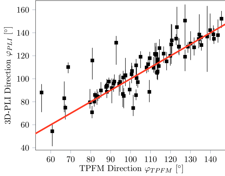
FIGURE E.4: Comparison of 3D-PLI and TPFM ground truth directions including 3D-PLI variability analysis. 3D-PLI directions were obtained from the GOROFI algorithm. The errorbars indicate the boundaries of the shortest interval which contains 67% of all samples. For reasons of clarity, only every third fiber bundle is plotted.
