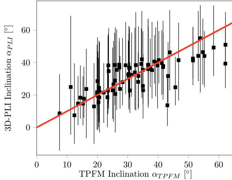
FIGURE E.5: Comparison of 3D-PLI and TPFM ground truth inclinations including 3D-PLI variability analysis. 3D-PLI inclinations were obtained from the GOROFI algorithm. The errorbars indicate the boundaries of the shortest interval which contains 67% of all samples. For reasons of clarity, only every third fiber bundle is plotted.
