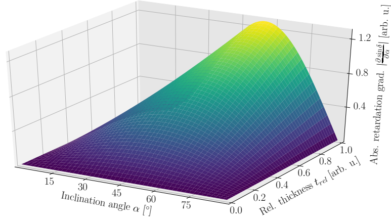
FIGURE 4.4: Absolute retardation gradient with respect to inclination \left| \frac{\partial \sin \delta}{\partial \alpha} \right| as a function of inclination and relative thickness t_{\text{rel}} .
