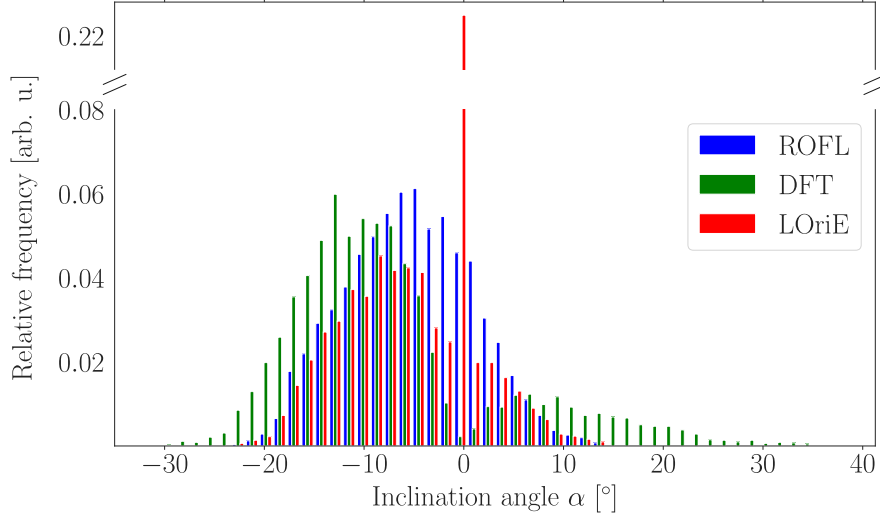
FIGURE 4.9: Inclination histograms for one ROI of in-plane oriented nerve fibers obtained from the ROFL, DFT and LOriE algorithms.
