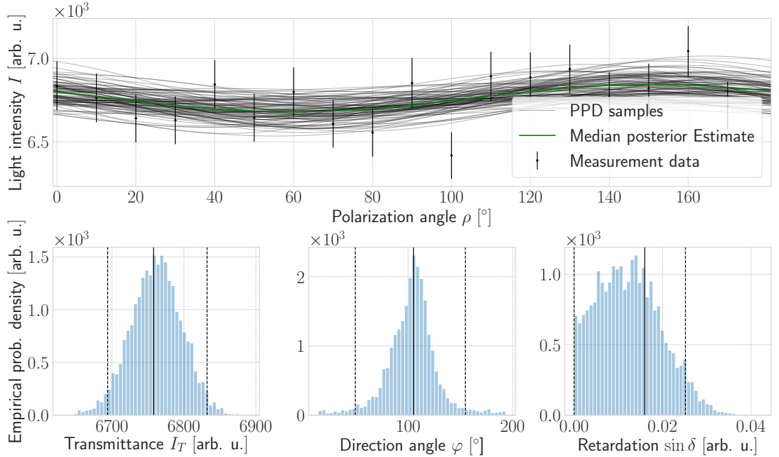
FIGURE 6.4: Results of the BAMBI framework for a grey matter pixel. The position of the pixel is pointed out by the red circle in Fig. 6.2. Top: measured light intensities and 100 samples of the posterior predictive distribution. Bottom: marginal distributions of transmittance, direction angle and retardation. Dashed lines indicate the boundaries of the 95% HPD intervals.
