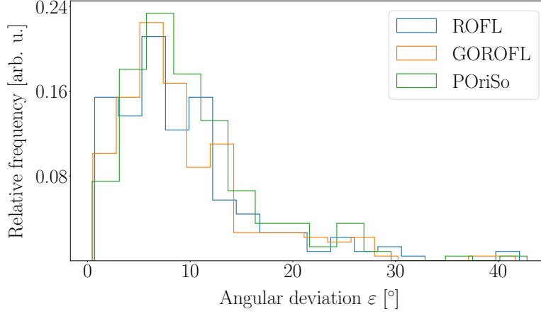
FIGURE 7.4: Histograms of angular deviations between TPFM fiber bundle orientations and 3D-PLI fiber bundle orientations computed by ROFL, POriSo and GOROFL.
