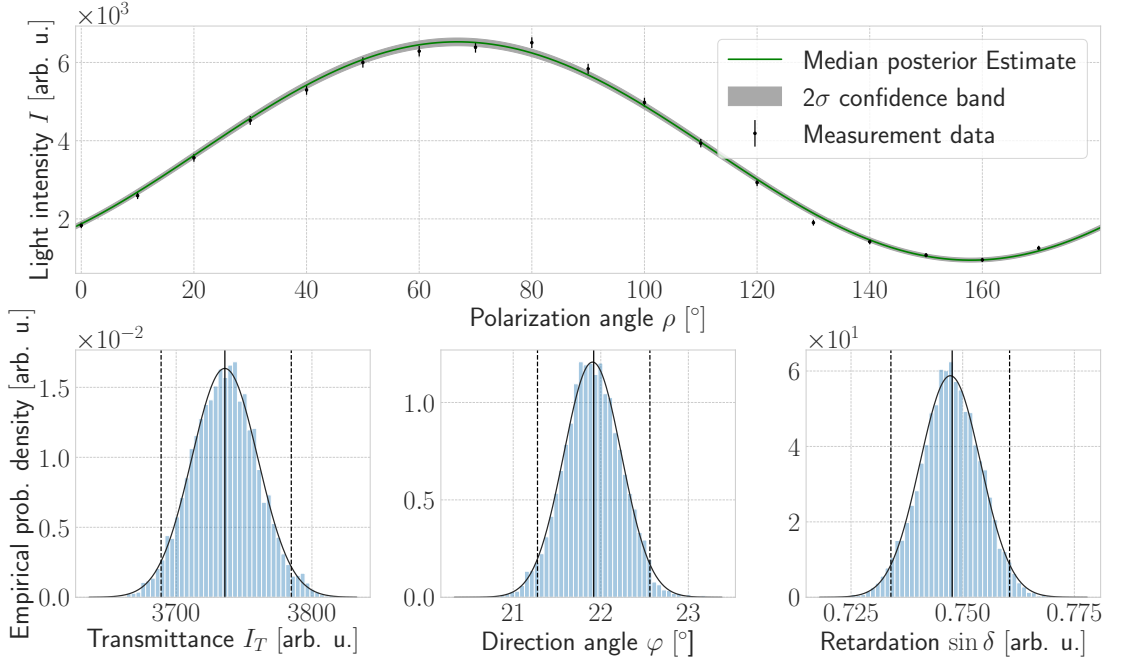
FIGURE 6.3: Results of the BAMBI framework for a white matter pixel. The position of the pixel is pointed out by the blue circle in Fig. 6.2. Top: measured light intensities and the 2\sigma confidence interval given by the 95% HPD interval of the posterior predictive distribution. Bottom: marginal distributions of transmittance, direction angle and retardation and normal distribution fit. Dashed lines indicate the boundaries of the 95% HPD interval.
