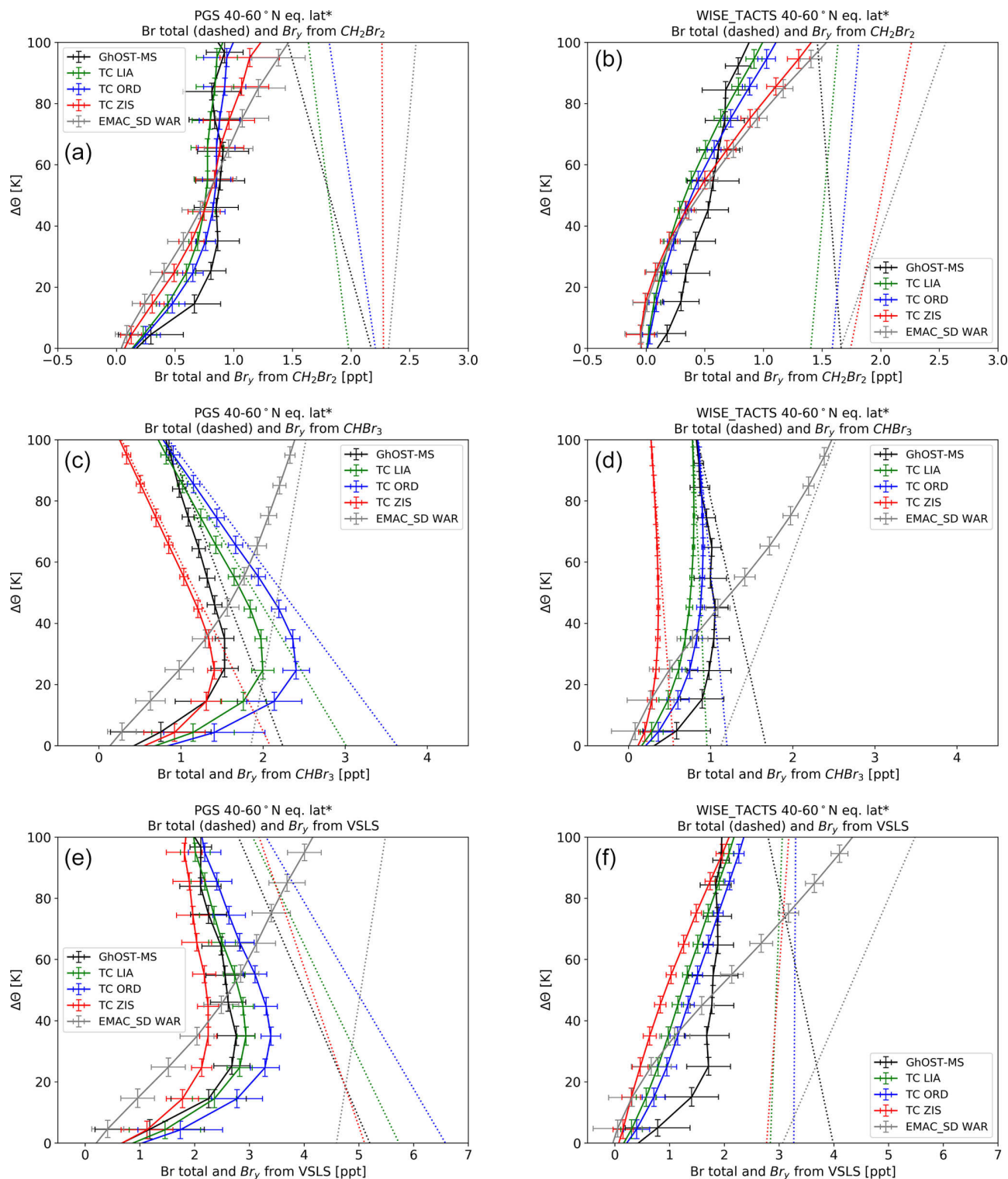
Figure 14. Vertical profiles of Br_y (solid lines) and total bromine (dotted lines) from CH_2Br_2 , CHBr_3 and total organic VSLs bromine averaged over 40\text{--}60^\circ of equivalent latitude* for the winter PGS campaign ( a , c , e , late December 2015 to March 2016) and the period from late summer to early fall ( b , d , f , WISE and TACTS campaigns) in comparison to model results from the TOMCAT and the EMAC model using different emission scenarios (see text for details on calculation of Br_y ). Total bromine is calculated from data at the tropical and extratropical tropopause and using assumptions about fractional input from these two source regions (see text for details). The data are displayed as a function of potential temperature above the tropopause. In the case when no model information on the tropopause altitude was available (TOMCAT), climatological tropopause values have been used (see text for details).
