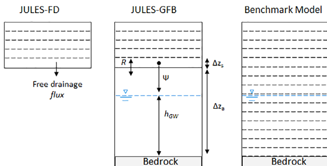
FIGURE 1 (a) Schematic overview of JULES-FD with the free drainage assumption, (b) JULES-GFB with the simplified groundwater representation and (c) the full 3-D hydrological model used as a benchmark (shown here as a 1-D column for simplicity)
