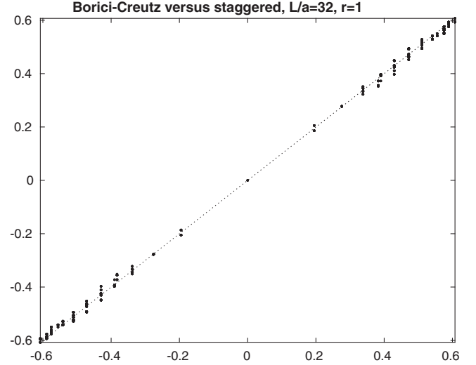
FIG. 11. Sorted free-field eigenvalues (with a twofold degeneracy removed) of the BC operator at r = 1 plotted versus sorted staggered eigenvalues (with a fourfold degeneracy removed). In both cases the imaginary part \text{Im}(\lambda) = \lambda/i at am = 0 is used, and plenty of degeneracies remain. The dotted line shows the identity for comparison.
