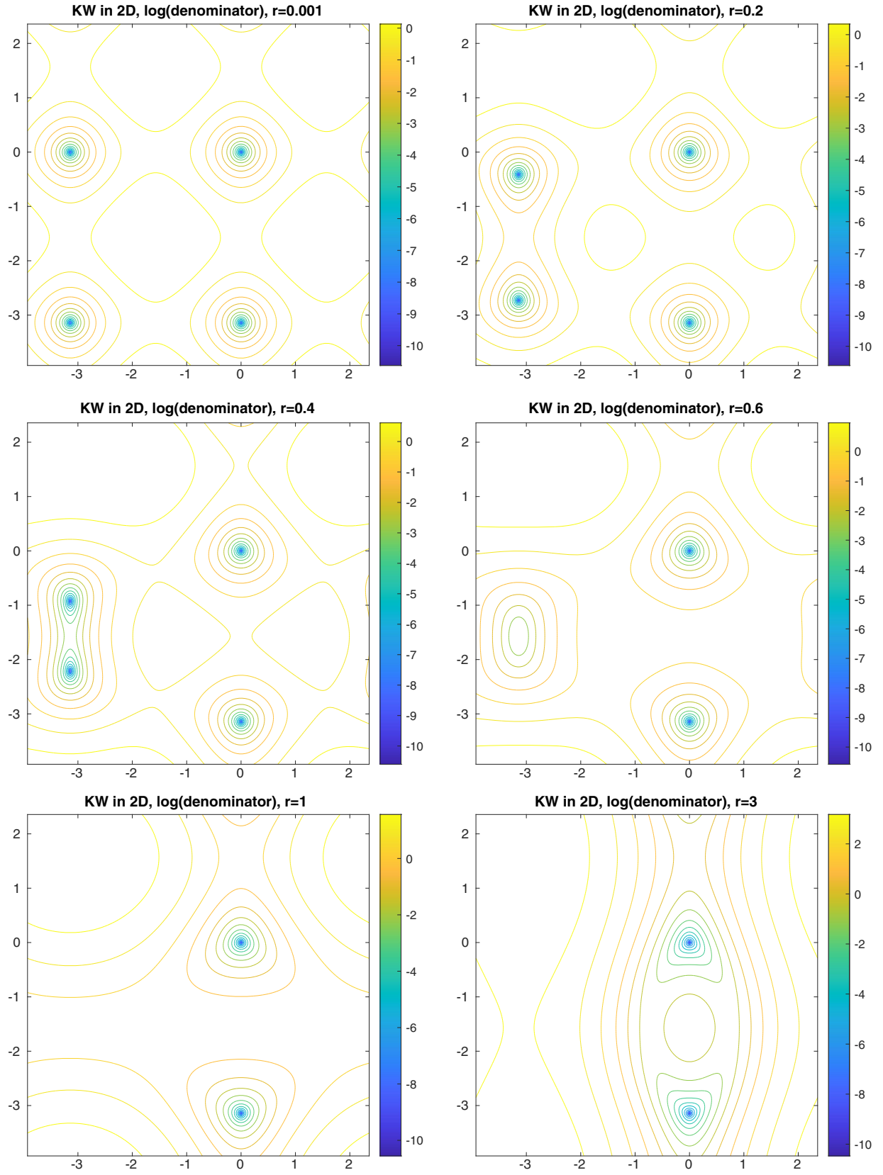
FIG. 13. Contour plots of the denominator of the KW propagator in d = 2 spacetime dimensions for r \in \{0.001, 0.2, 0.4, 0.6, 1, 3\} . Two poles annihilate at r = 1/2 .
