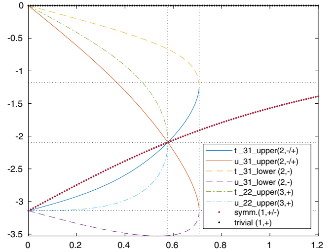
FIG. 15. Illustration of the free-field pole structure of the Borici-Creutz operator in d = 4 dimensions. Throughout, the momentum ap or aq is plotted as a function of the lifting parameter r . The full/dashed lines give 2\arctan(t), 2\arctan(u) with the 3-to-1 solutions t, u defined in the upper/lower line of (C20). The dash-dotted lines give 2\arctan(t), 2\arctan(u) with the 2-to-2 solutions t, u defined in the upper line of (C24). The lower line of that system interchanges t \leftrightarrow u , and would give the same graph. The fat-dotted lines indicate the symmetric solution -2\arctan(1/r) and the trivial solution. The horizontal dotted lines are at lattice momentum -3\pi/8, -2\pi/3 , and -\pi , respectively. The vertical dotted lines are at r = 1/\sqrt{2} , and r = 1/\sqrt{3} , respectively. In d = 2 dimensions all 3-to-1 paired solutions would be absent, the dash-dotted curve would refer to (C9), and the fat-dotted curves would be unchanged.
