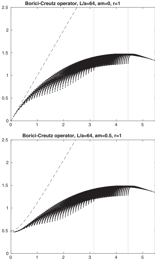
FIG. 8. Same as Fig. 1, but for the BC operator at r = 1 .
