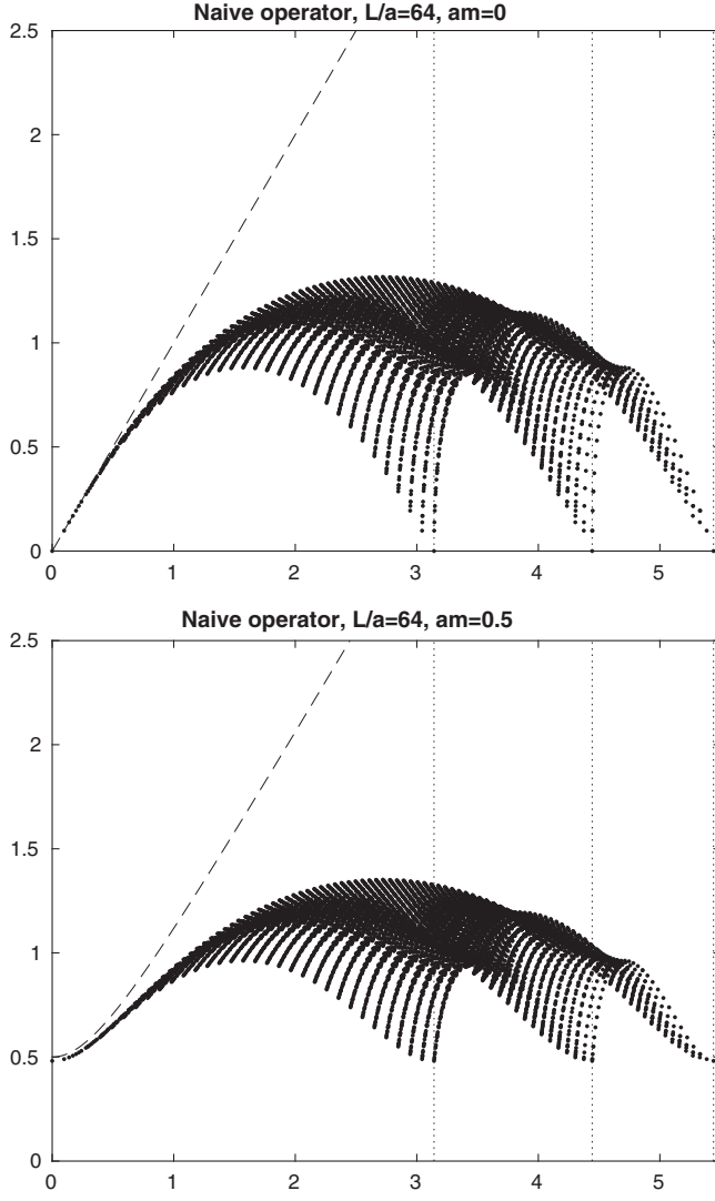
FIG. 1. Free-field dispersion relation aE versus a|\vec{p}| of the naive Dirac operator at am = 0 and am = 0.5 . The dashed curves give the continuum dispersion relations, and the vertical lines show the end of the Brillouin zone in the (1,0,0) , (1,1,0) , and (1,1,1) directions, respectively.
