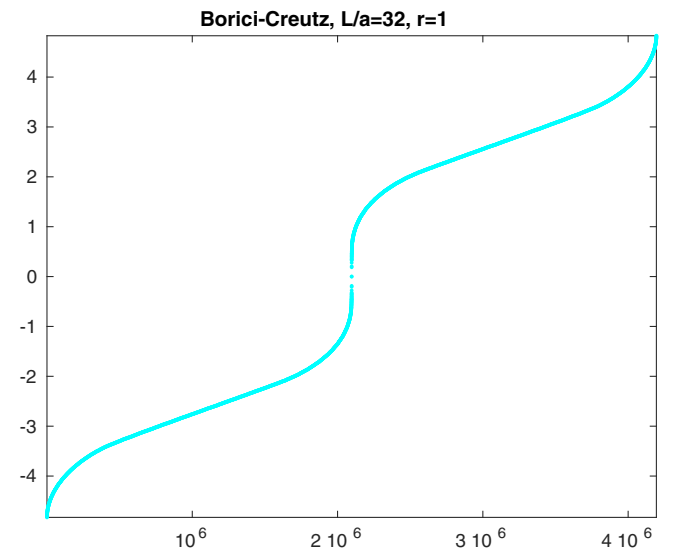
FIG. 9. Free-field eigenvalue spectrum of the BC operator at r = 1 . The imaginary part is plotted against the index.
