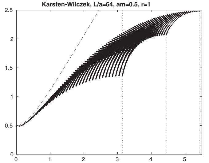
FIG. 4. Same as Fig. 1, but for the KW operator at r = 1 .
