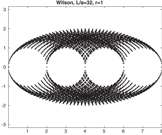
FIG. 3. Free-field Wilson eigenvalue spectrum at r = 1 in the complex plane.
