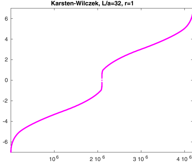
FIG. 5. Free-field eigenvalue spectrum of the KW operator at r = 1 . The imaginary part is plotted against the index.
