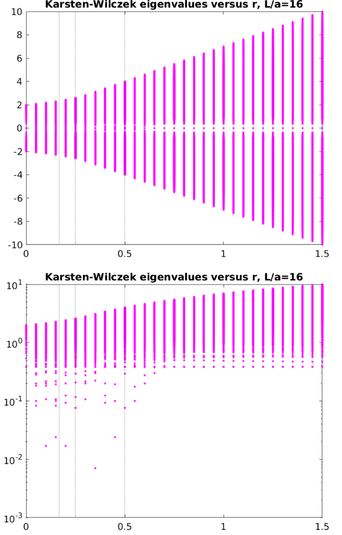
FIG. 6. Imaginary part of the free eigenvalues of the KW operator in linear and logarithmic representation (for the upper half-spectrum) versus the lifting parameter r . The vertical lines at r = 1/6, 1/4, 1/2 mark the transitions to 14, 8, and 2 species, respectively.
