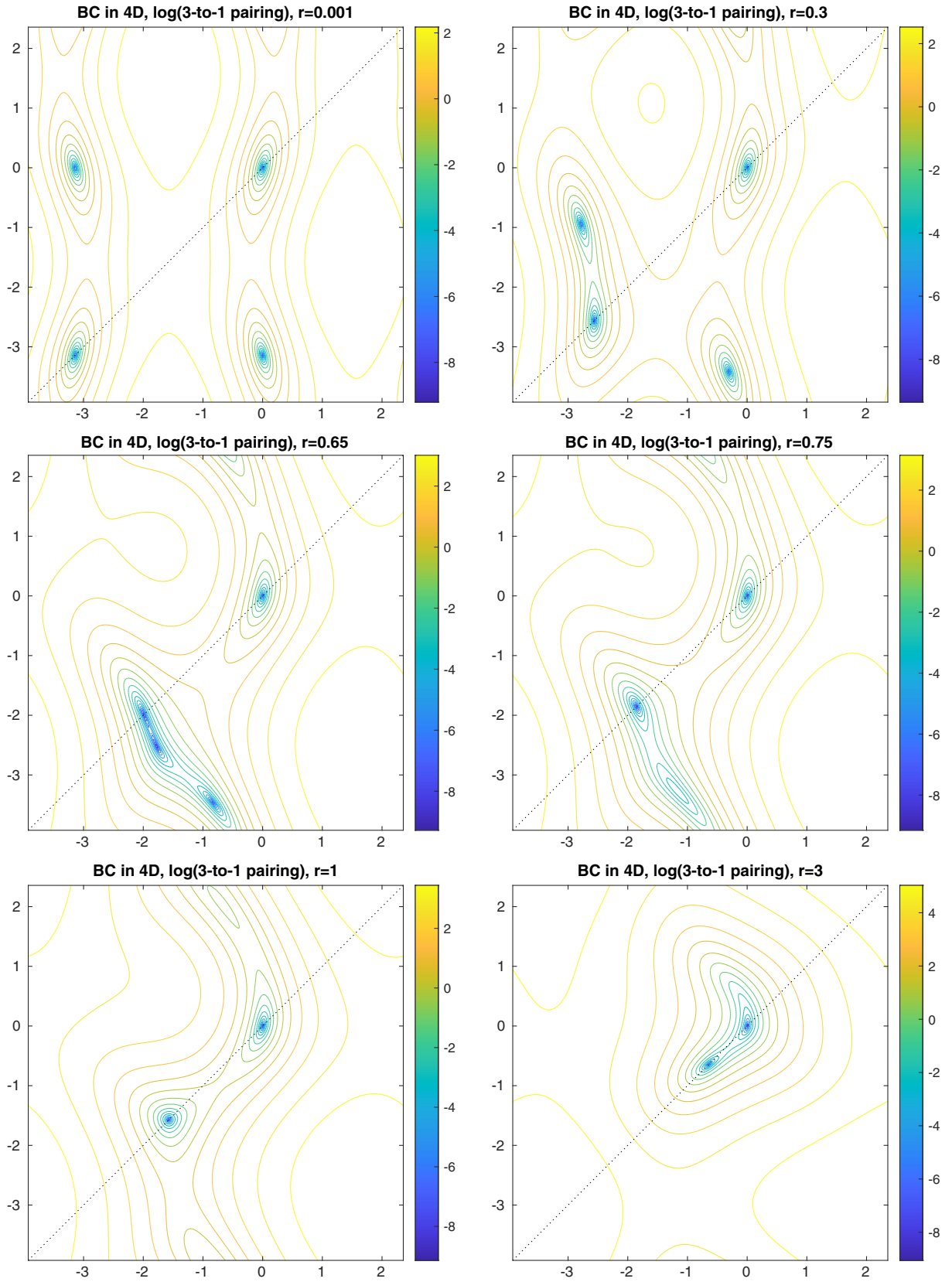
FIG. 16. Contour plots for the solutions to (C17) for r \in \{0.001, 0.3, 0.65, 0.75, 1, 3\} . There are touch- and endpoints at r = 1/\sqrt{3} \simeq 0.57735 , and r = 1/\sqrt{2} = 0.70711 . See text for details.
