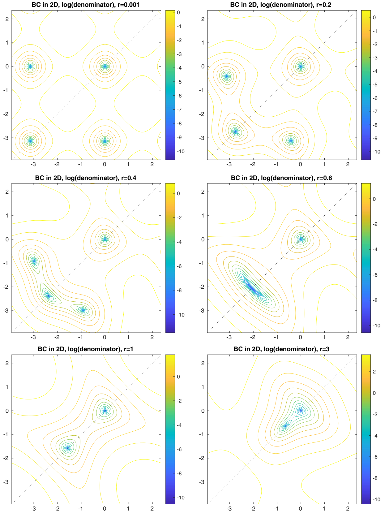
FIG. 14. Contour plots of the denominator of the BC propagator in d = 2 spacetime dimensions for r \in \{0.001, 0.2, 0.4, 0.6, 1, 3\} . Three poles merge into one at r = 1/\sqrt{3} \approx 0.57735 .
