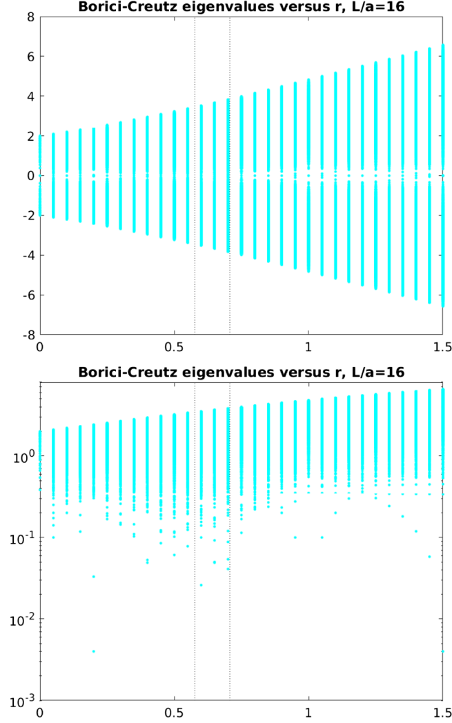
FIG. 10. Imaginary part of the free eigenvalues of the BC operator in linear and logarithmic representation (for the upper half-spectrum) versus the lifting parameter r . The vertical lines at r = 1/\sqrt{3} and 1/\sqrt{2} mark the transitions to ten and two species, respectively.
