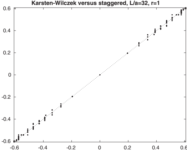
FIG. 7. Sorted free-field eigenvalues (with a twofold degeneracy removed) of the KW operator at r = 1 plotted versus sorted staggered eigenvalues (with a fourfold degeneracy removed). In both cases the imaginary part \text{Im}(\lambda) = \lambda/i at am = 0 is used, and plenty of degeneracies remain. The dotted line shows the identity for comparison.
