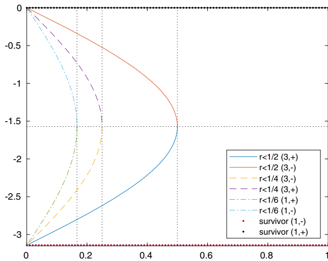
FIG. 12. Illustration of the free-field pole structure of the Karsten-Wilczek operator in d = 4 dimensions. The momentum ap_4 is always plotted as a function of the parameter r . The threefold degenerate solution that emerges from (0, 0, \pi) , (0, \pi, 0) , or (\pi, 0, 0) , together with ap_4 = \pm\pi , has correct chirality. It annihilates, at r = 1/2 , with the threefold degenerate counterpart that emerges from ap_4 = 0 with opposite chirality. The threefold degenerate solution that emerges from (0, \pi, \pi) , (\pi, 0, \pi) , (\pi, \pi, 0) , together with ap_4 = \pm\pi , has opposite chirality. It annihilates, at r = 1/4 , with the threefold degenerate counterpart that emerges from ap_4 = 0 with correct chirality. The nondegenerate solution that emerges from (\pi, \pi, \pi) , together with ap_4 = \pm\pi , has correct chirality. It annihilates, at r = 1/6 , with the nondegenerate counterpart that emerges from ap_4 = 0 with opposite chirality. The nondegenerate solution that emerges from (0, 0, 0) and ap_4 = \pm\pi has opposite chirality and lives for any r . The nondegenerate solution stemming from the same spatial momentum, but with ap_4 = 0 , has correct chirality and lives for any r .
