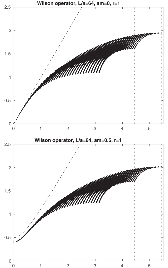
FIG. 2. Same as Fig. 1, but for the Wilson operator at r = 1 .
