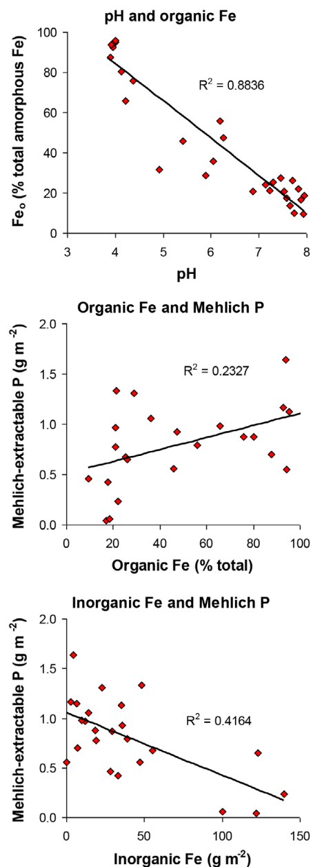
Fig. 6. Relationships between different forms of Fe and P: pH and organic Fe, as percentage of total amorphous Fe, the percentage of organic Fe and Mehlich-extractable P, and the amount of inorganic Fe and Mehlich-extractable P. All correlations were significant ( P < 0.05 ).
