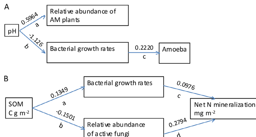
Fig. 13. D-separation tests conducted as a form of piecewise structural equation modeling. Model A tested whether pH could be a causal factor to the relative abundance of arbuscular mycorrhizal (AM) plants (a) and bacterial growth rates (b), measured as incorporation of thymidine ( \text{pmol} \cdot \text{g}^{-1} \cdot \text{h}^{-1} ), which in turn could affect numbers of amoeba in the soil (c). Model B tested whether soil organic matter (SOM) could be a causal factor for bacterial growth rates (a) and the relative abundance of active fungi (b), which both in turn could affect net N mineralization (c and d). Both models were valid as cause and effect model (model A: Fisher's C test: 4.490854, df: 4, P : 0.34633; model B: Fisher's C test: 2.938, df: 4, P : 0.568).
