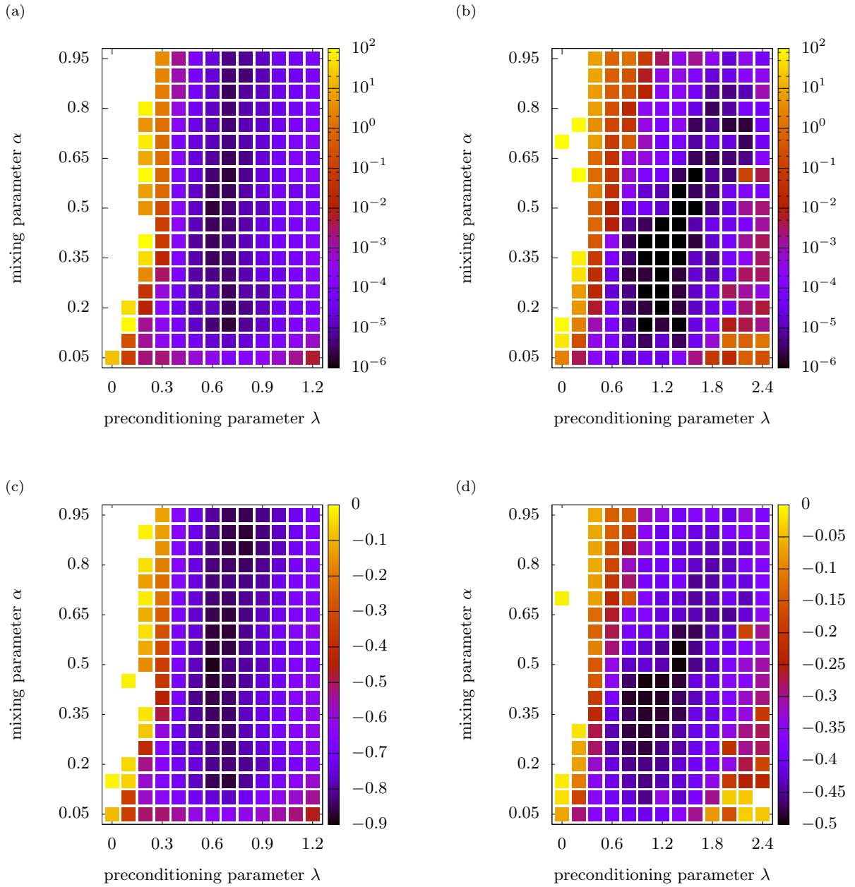
FIG. 3. The distance of \rho_{\text{out}} and \rho_{\text{in}} in \text{me}/a_0^3 for a number of mixing parameters \alpha and a number of Kerker parameters \lambda for the 19-atom system of (a) Cu after 20 and (b) Fe after 35 iterations. The slope of a linear fit of the logarithmically plotted distance for the same systems of (c) Cu and (d) Fe. The color codes in the slope plots are restricted to values \leq 0 . White spots mean that the iteration did not converge within (a) 20, (b) 35, (c) 30, and (d) 50 iterations, respectively.
