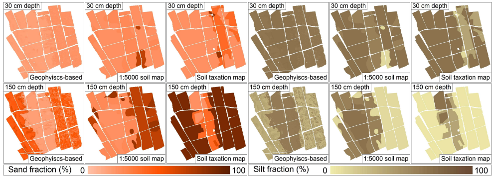
Figure 33: percentages of sand (orange color scale) and silt (brown color scale) at 30 cm and at 150 cm in the three soil maps.
