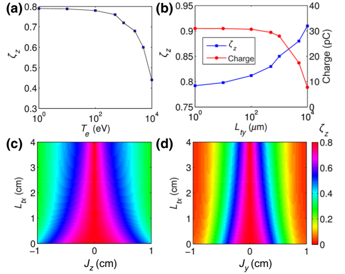
FIG. 5. (a) Polarization along the z axis as a function of initial electron temperature. (b) Polarization (blue squares) and selecting charge (red circles) as a function of the transverse size (along the y axis) of the filter L_{ty} . The polarization as a function of longitudinal thickness (along the x axis) L_{tx} and drive-beam jitter in the z direction ( j_y = 0 ) (c) and in the y direction ( j_z = 0 ) (d). The target is set 50 cm from the filter. The selecting angle \Delta\phi = \pi/2 , while the other simulation parameters are the same as in Fig. 1.
