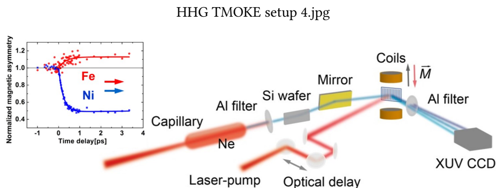
Figure 8: Experimental setup for element-selective spin dynamics. The laser pump and XUV probe beams are derived from a single laser amplifier. The XUV light propagates in vacuum and contains a spectrum of photons with energies between 20 and 72 eV. The inset (left) shows time-resolved magnetization of the Fe and Ni layers in the Fe/Ru/Ni trilayer. The magnetic asymmetry at the Fe 3p absorption edge anomalously increases for the parallel magnetic orientation of Ni and Fe layers thus confirming the presence of laser-driven spin superdiffusion from Ni to Fe layer.
