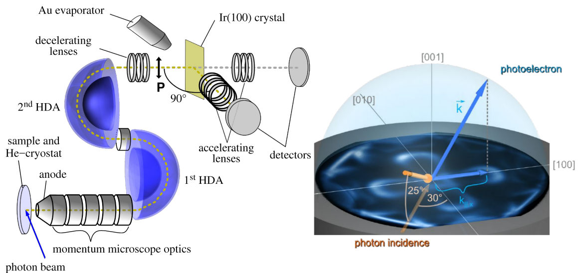
Figure 13: Left side : Working principle of a spin-resolving electron momentum microscope (SPEMM) consisting of the imaging electron optics, electrostatic energy filter, imaging spin-filter with Ir(100) mirror, and detectors (Tusche et al., 2015). Right side : Emission of photoelectrons into the complete half-space above the sample surface and the related intensity distribution in reciprocal space. The SPEMM experiment collects all photoelectrons simultaneously.
