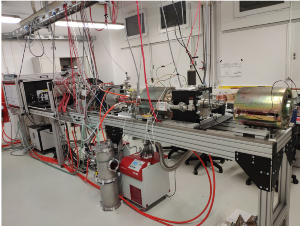
Figure 14: Photo of JüSPARC_MIRA and the Lamb-shift polarimeter.
