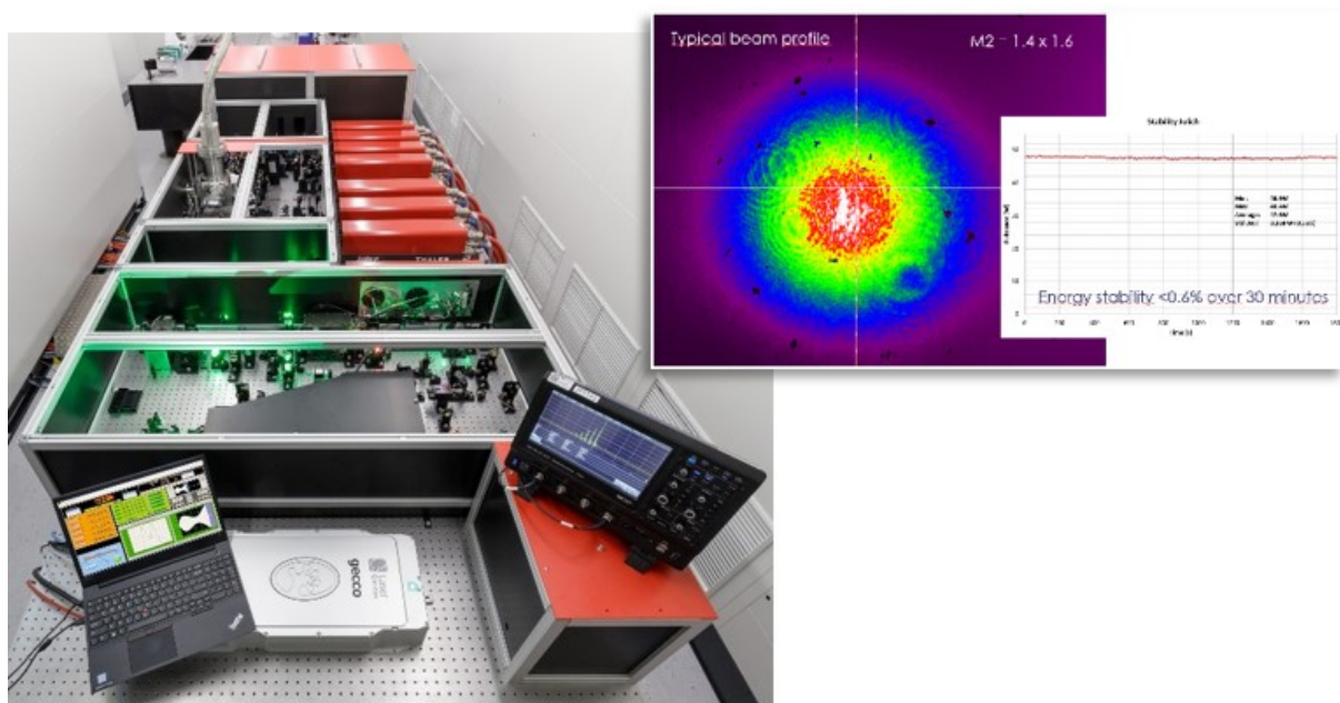
Figure 4: Overview of the 1.3 TW two-stage amplifier built by THALES, consisting of an oscillator (front), the first amplification stage (front), the second amplification stage with cryocooled Ti:Sapphire crystal (middle left), eight pump lasers (middle right, red) and the compressor unit (far side). The typical beam profile and output energy stability are shown on the right.
