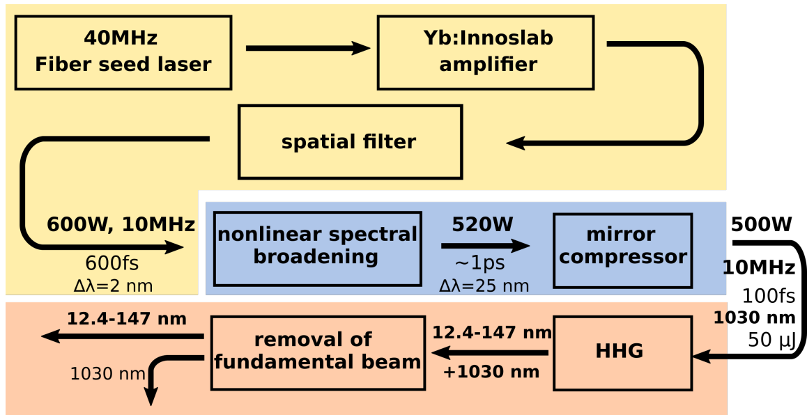
Figure 10: Schematic setup of JuSPARC_SIRIUS for spin- and time-resolved electron momentum microscopy, which consist of Innoslab amplifier (shaded yellow region) (Russbueltd et al., 2015), nonlinear compression using multi-pass cell (Weitenberg et al., 2017) (shaded blue region) and XUV-initiated HHG (shaded orange region).
