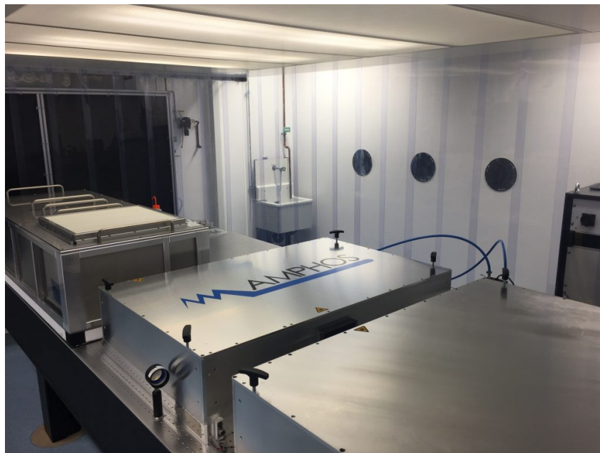
Figure 11: Photo of JuSPARC_SIRIUS laser system. The high-power laser is operated under clean room conditions with multi-stage air filter systems, producing a low-turbulence laminar airflow to create a particle-free environment.
