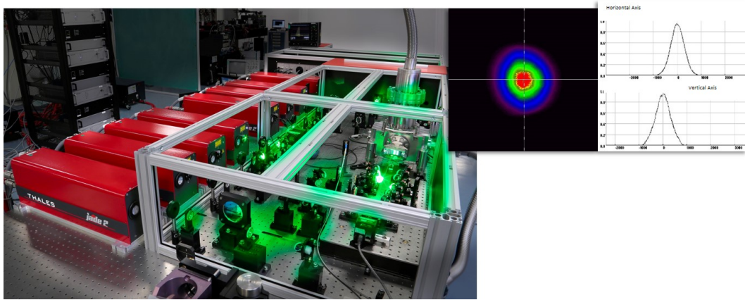
Figure 5: The block of eight pump lasers and the second amplification stage. The first pump laser is used to pump the first amplification stage, while the remaining seven pump lasers are employed for pumping the cryo-cooled Ti:Sapphire crystal of the second amplification stage. The typical beam profile of a Jade 2 pump laser is shown on the right.
