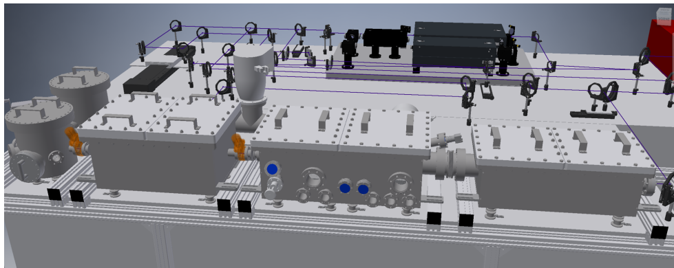
Figure 7: HHG beamline for high-energy photon and electron scattering experiments. From right to left: focusing chamber, HHG source chamber containing the gas cell, monochromator, and experiment and detection chambers. The high-energy photon beam is generated and guided inside vacuum to avoid scattering in air.
