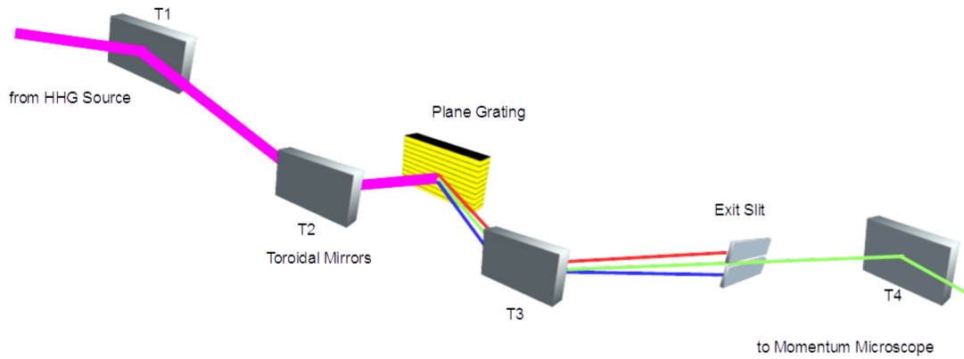
Figure 12: JuSPARC_SIRIUS beamline. The XUV light, produced in the HHG process for photoemission, is monochromatized and transported to the momentum microscope.
