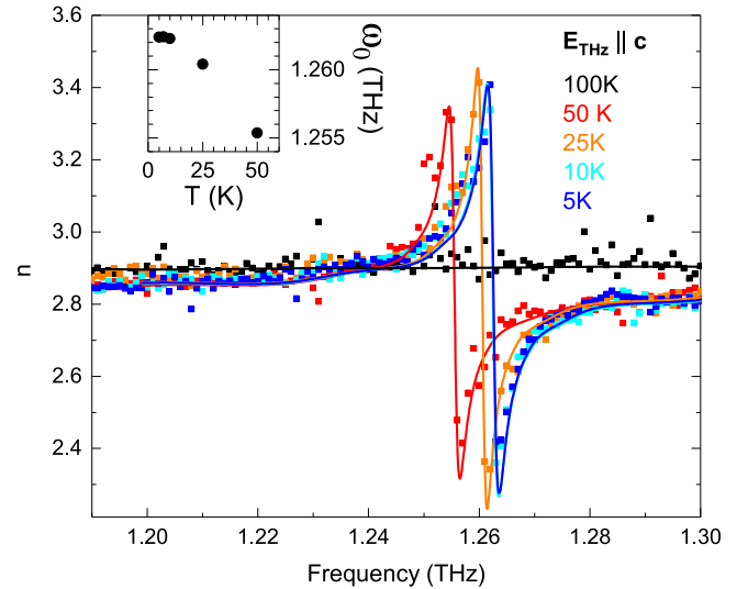
FIG. 3. Refractive index of (\text{NH}_4)_2[\text{FeCl}_5(\text{H}_2\text{O})] for polarization \mathbf{E} \parallel \mathbf{c} . Below T_S , we observe the appearance of a mode at about 1.26 THz, which we attribute to a libration of the \text{NH}_4^+ groups. Symbols show the experimental results, solid lines depict fits using a Lorentz oscillator. The inset resolves the temperature dependence of the eigenfrequency of this mode.
