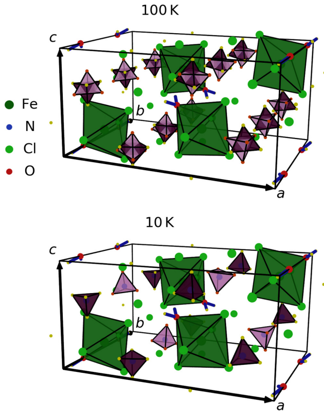
FIG. 6. Crystal structure of (\text{ND}_4)_2[\text{FeCl}_5(\text{D}_2\text{O})] at 100 K (top) and 10 K (bottom). \text{ND}_4^+ tetrahedra of the same shading are symmetry equivalent.
