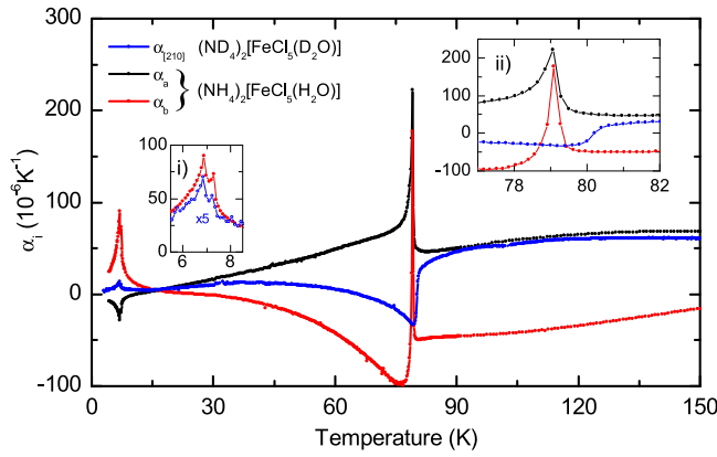
FIG. 4. Thermal expansion \alpha_{[210]} measured along the [2\ 1\ 0] direction of (\text{ND}_4)_2[\text{FeCl}_5(\text{D}_2\text{O})] in comparison to the a - and b -axis expansions of (\text{NH}_4)_2[\text{FeCl}_5(\text{H}_2\text{O})] from Ref. [15]. An enlarged view of the low-temperature transitions is shown in inset (i) with \alpha_{[210]} multiplied by a factor of 5 to allow for a better comparison. Inset (ii) enlarges the structural transition-temperature regime.
