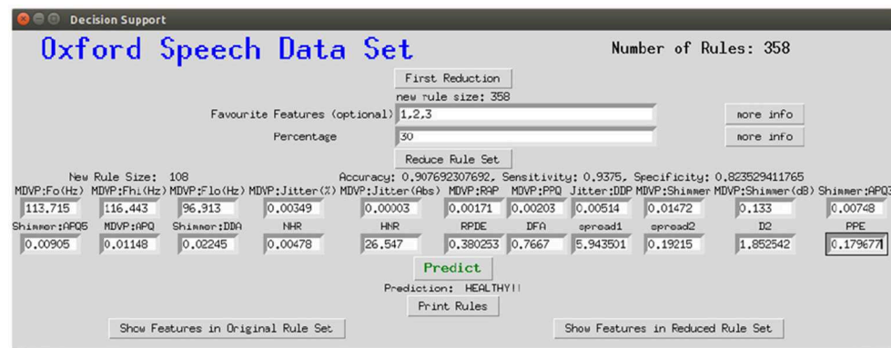
FIGURE 8 | Graphical interface for the clinical decision support system, here applied to the Speech Data Set.
