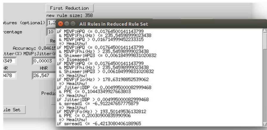
FIGURE 9 | Displaying all rules that remained in the reduced rule set.
