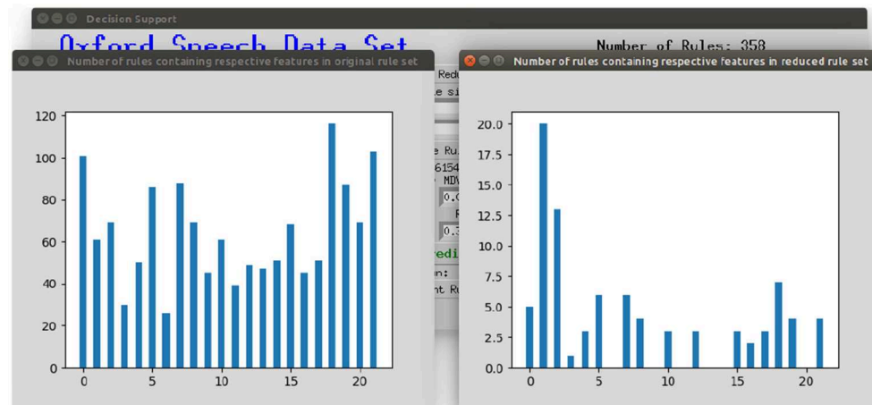
FIGURE 10 | Displaying the number of rules containing the respective feature in the original rule set and the current reduced rule set.
