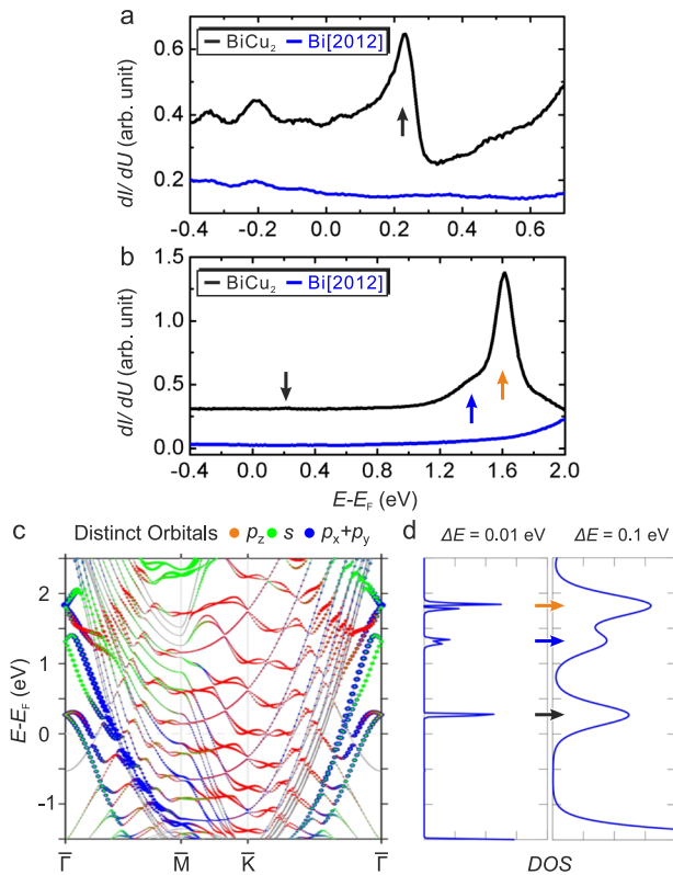
Fig. 2 Electronic structures of unoccupied Rashba spin-split bands. From a , an asymmetric peak at 0.23 V has been resolved from dI/dU curve on \text{BiCu}_2 (black line). In contrast to \text{BiCu}_2 , the dI/dU curve on \text{Bi}[2012] is rather featureless (blue line). (stabilization parameters: U = +0.7 V, I = 1.0 nA, T = 4.5 K). From b , a pronounced peak at 1.6 V as indicated by red arrow together with a shoulder at 1.4 V (blue arrow) has been observed on \text{BiCu}_2 , but no characteristic features can be observed from the dI/dU curve taken at \text{Bi}[2012] . (stabilization parameters: U = +2.0 V, I = 1.0 nA, T = 4.5 K). c Orbital-decomposed band structure of the \text{BiCu}_2 surface. The red, green, and blue spheres indicate, respectively, the p_z , s , and p_x + p_y orbital contributions. DOS from band edges and the nearby crossing point of unoccupied Rashba bands resulting in the peak positions in d . The crossing points of the Rashba bands at \bar{\Gamma} correspond to the peak positions in d . d The DOS integrated over the zone-center region near the \bar{\Gamma} point for comparison with our scanning tunneling spectroscopy (STS) results. The left (right) panel shows DOS with \Delta E = 0.01 eV ( \Delta E = 0.1 eV) broadening.
